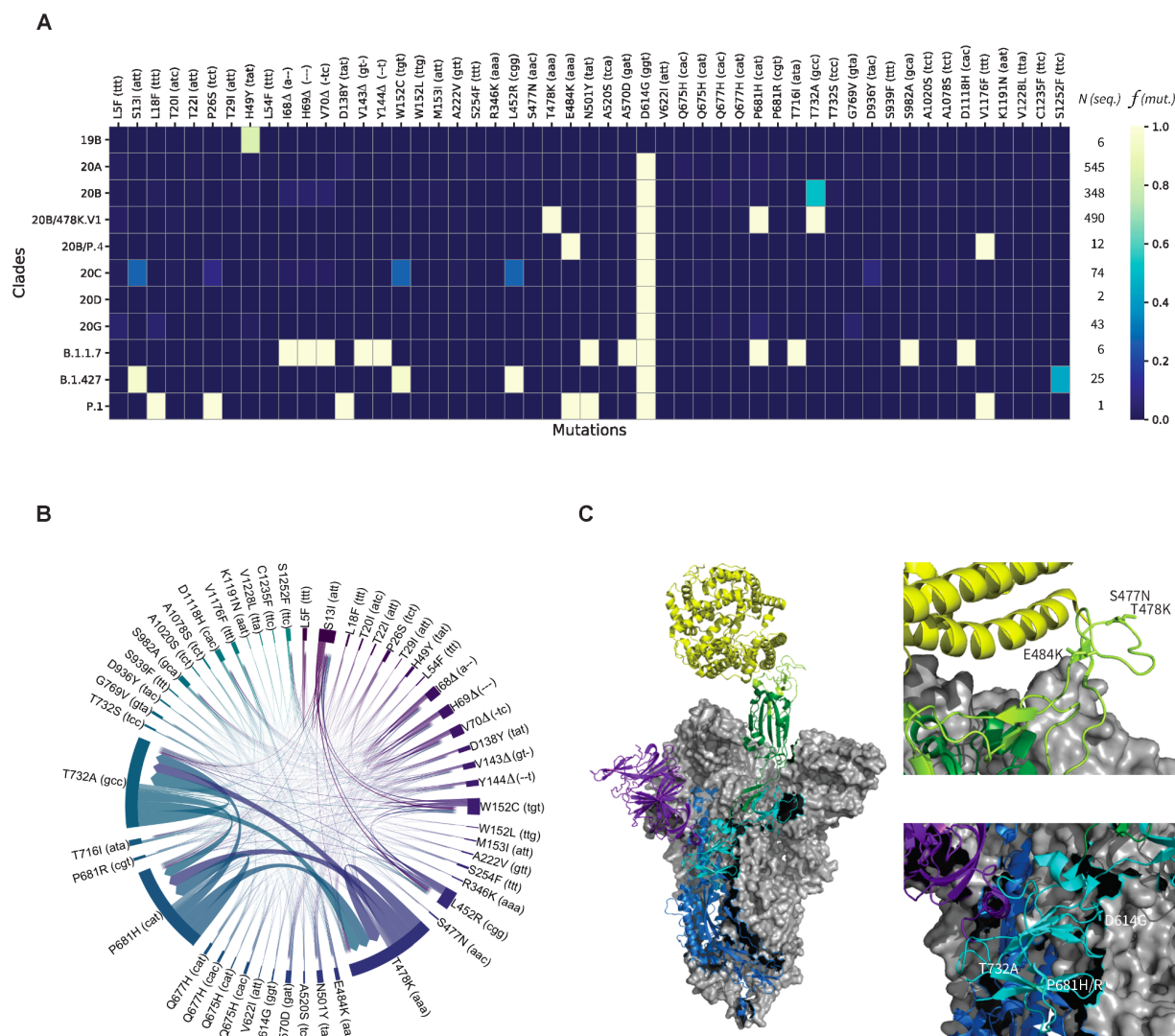
Figure 2. Systematic sequence/structure analysis of Spike protein mutations of concerns. A ) The heatmap highlights relative frequencies f for 51 important mutations (out of 315) across 1552 viral genomes arranged in 11 clades (19B, 20A-D, 20B/478K.V1, 20B/P.4, 20G, B.1.1.7, B.1.427, P.1). N indicates the number of available genome sequences per clade. See supplementary Figure S5 for a heatmap including all mutations. B ) The chord diagram displays the covariances between the 51 most frequent mutations. The thickness of the arrows denotes the strength of a covariance. C ) Left - Electron Microscopy structure (PDB:7A94 ref) of the trimeric Spike (S) glycoprotein of SARS-CoV-2 bound to one Angiotensin-Converting Enzyme-2 (ACE2, yellow). Two chains of the viral protein are shown in gray surfaces. The third chain comprises the N-terminal domain (purple), the S1 (cyan) and S2 (blue) protein subdomains, the Receptor-
