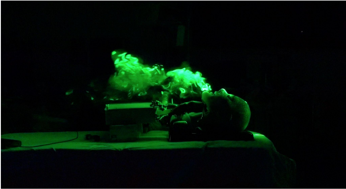
Figure 2: Patient position re-oriented to be located at the edge of the laminar flow, allowing the proceduralist for AGP to stand directly under the clean upstream flow. Laser image pre-data processing, at midline in the Sagittal plane, showing plume dispersing caudad, away from the HCW.
