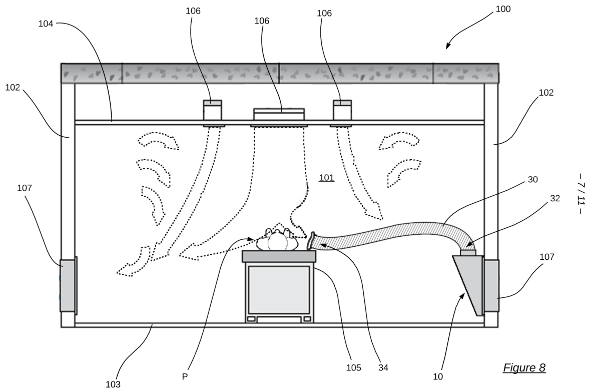
Supplementary Figure 8: Schematic for RIVET setup.
