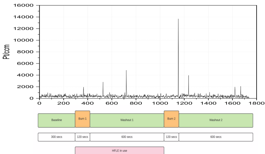
Supplementary Figure 7: Particle counts throughout the test. Locations A-D
