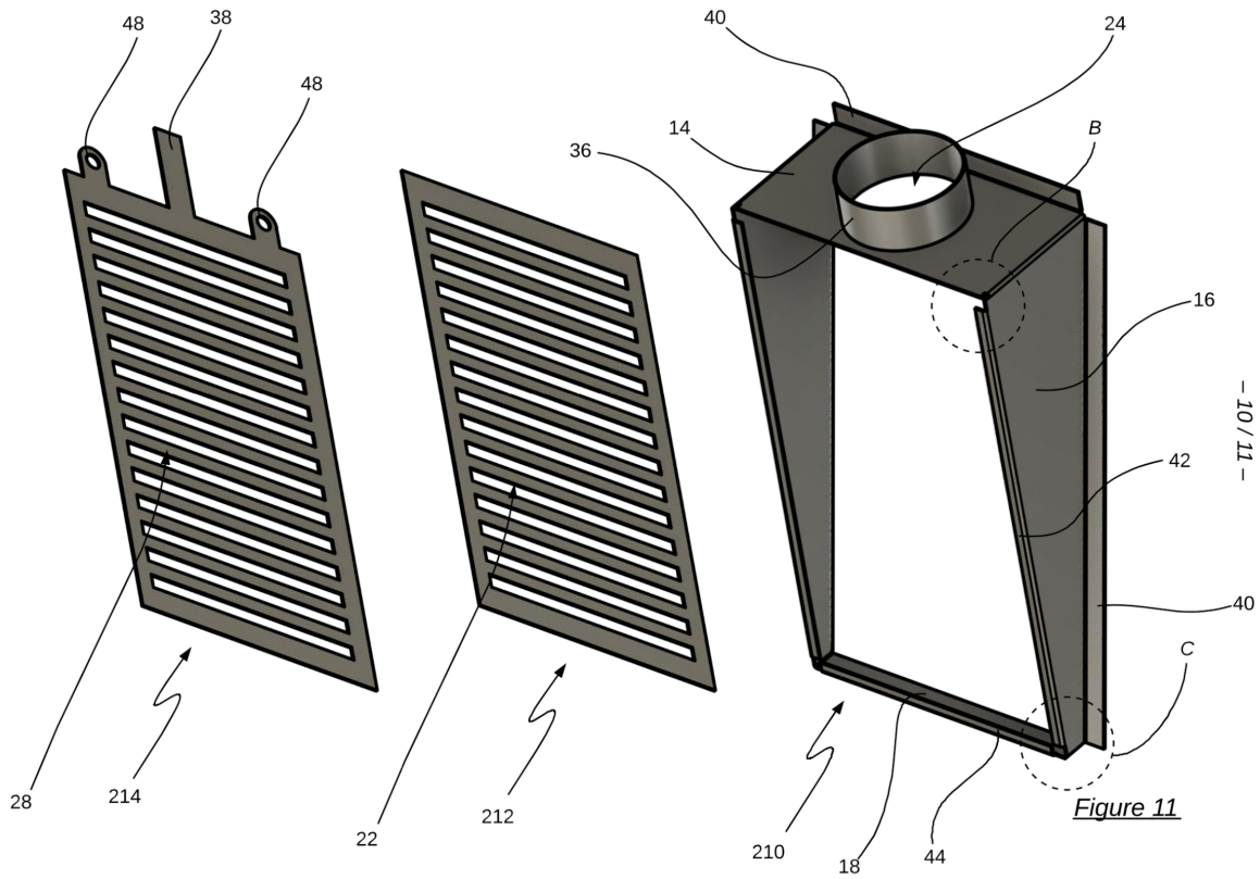
Supplementary Figure 9: Schematic for RIVET Exhaust vent cover version 2.0. Showing sliding louvre system, and hose attachment
