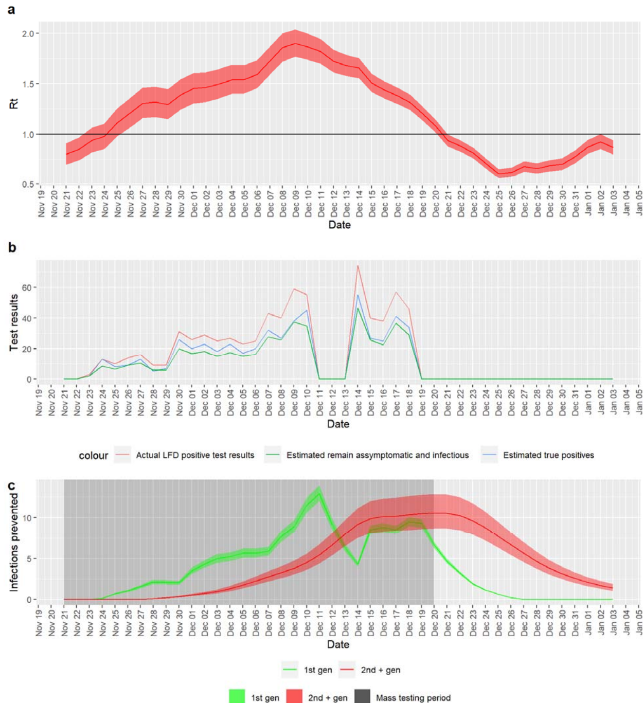
Figure 2: (a) Estimated R_t in Merthyr Tydfil over the testing period. (b) Positive lateral flow test results from community testing pilot in Merthyr Tydfil, with estimates for true positives and proportion remaining asymptomatic. Note that missing data in the weekend of 11th to 13th December is due to temporary suspension of the mass testing on these dates. (c) Daily estimates of 1st generation and 2nd + higher generation infections prevented
