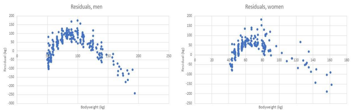
Figure 3A-B. Residuals of the models fit above, using doping test status as a binomial factor. The residuals are not normally distributed, but positive for the middleweight classes, and negative for the extremes of body weight. An allometric model is not a suitable system for adjusting powerlifting
