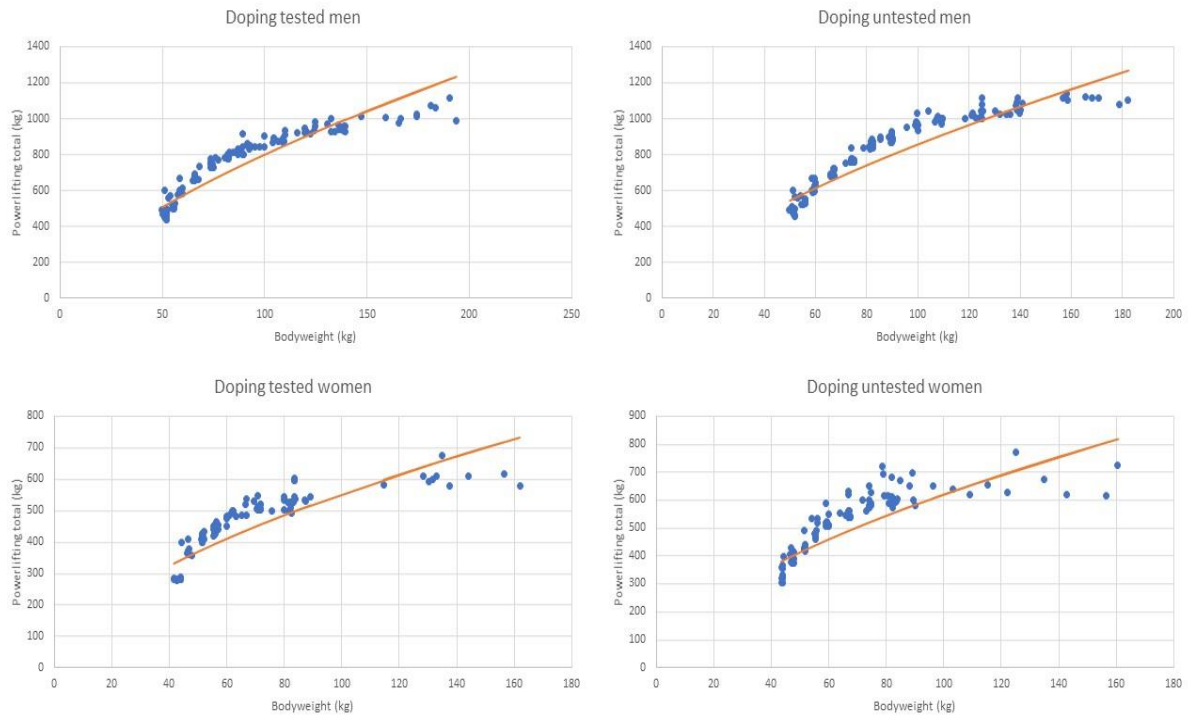
Figure 2A-D. The fit allometric prediction functions plotted against the powerlifting results.
