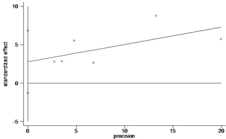
Egger's publication bias plot
