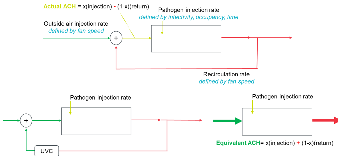
Fig. 1: Equivalent ACH (eACH) as it relates to fresh-air injection rate
