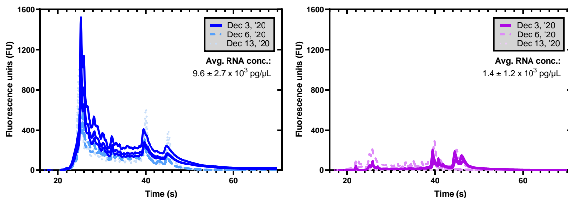
Figure 3: Electropherograms for samples from the lagoon and the pumping chamber, showing drastic differences in the RNA profiles. Total RNA concentrations were calculated using Agilent's 2100 Expert software (version B.02.10.SI764).
