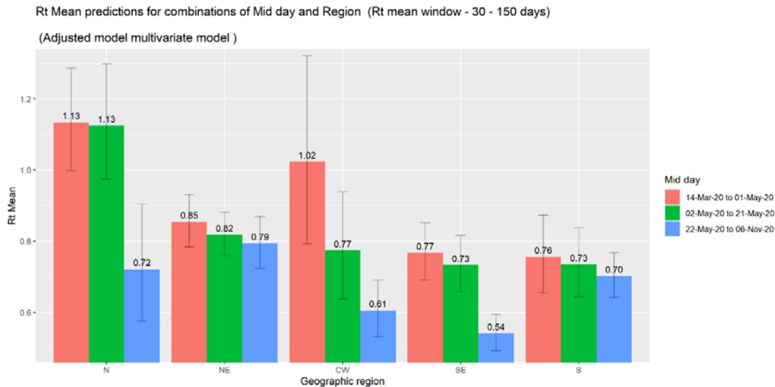
Figure 4 Estimated marginal mean values of R_t mean in the final adjusted multivariate linear regression model*.
