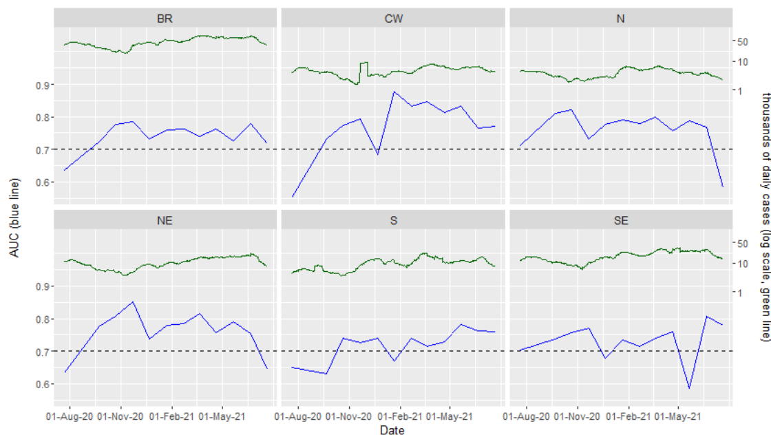
Figure 5. Area under the curve (AUC) for prediction of a new maximum incidence in the following 30 days (left vertical axis, blue line) against calendar time (horizontal axis). The daily number of incident cases (rolling fortnightly average) is shown in the green line, right axis. The dashed line shows the lower end of the range 0.70-0.90. There is one panel for each region (Central-West, North, North-East, South and South-East), with the “BR” panel showing all Brazil.
