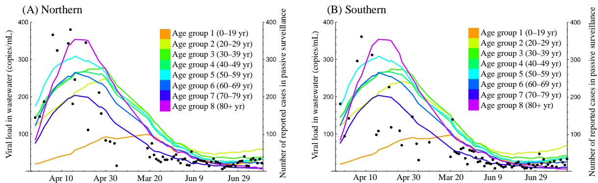
131 Fig. 1. Comparison between viral load in wastewater and the number of reported cases per age group in 132 passive surveillance. Dots show viral load in wastewater sampled in the treatment plant's (A) northern and 133 (B) southern area. Solid lines show the two-week moving average of the number of reported cases per age 134 group in passive surveillance, with color representing age group. 135
