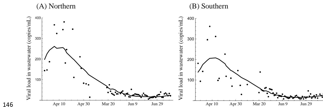
147 Fig. 2. Model fittings to the viral load in wastewater sampled in the (A) northern and (B) southern areas. 148 Solid lines show the model prediction and dots show the viral load in wastewater.
