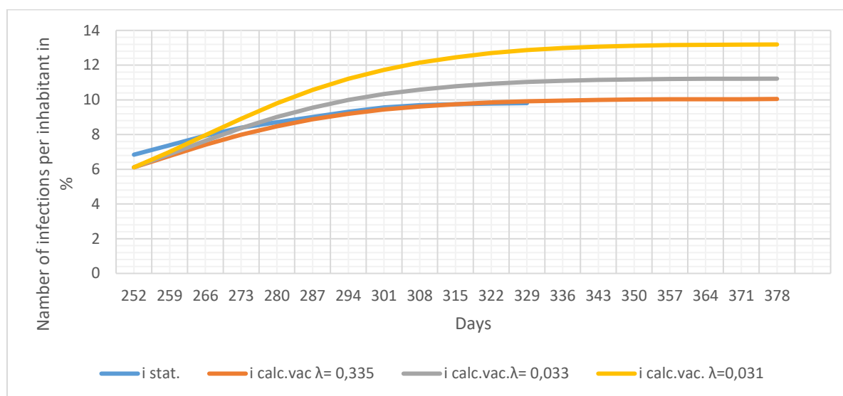
Fig. 3: Epidemic development during the vaccination period under different lockdown conditions
