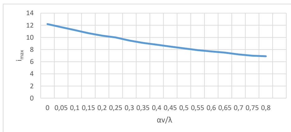
Fig. 2: Effect of vaccination rate on the intensity of epidemic growth
