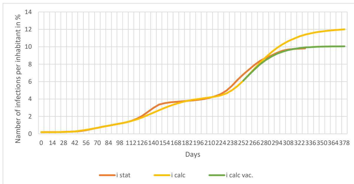
Fig.1: Development of the epidemic in Israel
