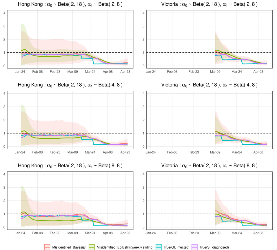
Fig 2. Estimations of local time-varying reproduction numbers in simulated epidemics for Hong Kong and Victoria under three sets of error misidentification rates: \alpha_0 \sim \text{Beta}(2, 18) , and \alpha_1 \sim \text{Beta}(2, 8) , \text{Beta}(4, 8) , or \text{Beta}(8, 8) . The error bands are the averages of 95% credible intervals over 1,000 trials. Note that the differences between the blue curve ( R_*^{\text{local}}(t) ) and the purple curve ( R^{\text{local}}(t) ) are due to the differences among infected dates, symptom onset dates, diagnosed dates.
