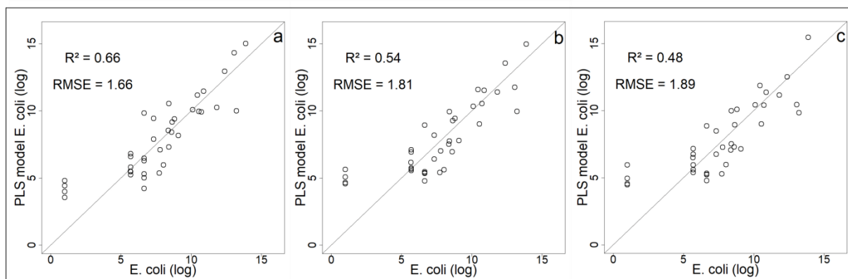
Fig 8. Comparison of models' predictions with observed E. coli (log values) (a) PLS model with all environmental variables and all components; (b) PLS model with NIR band, SPM and Weekly rainfall and all components; (c) PLS model with satellite variables only (NIR band and Weekly rainfall) and all components
