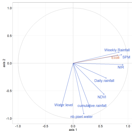
Fig 7. Correlation circle of partial least squares (PLS) regression, illustrating relationships between predictor variables (blue), E. coli (orange) and the two first PLS components (first component on the x-axis, second one on the y-axis).
