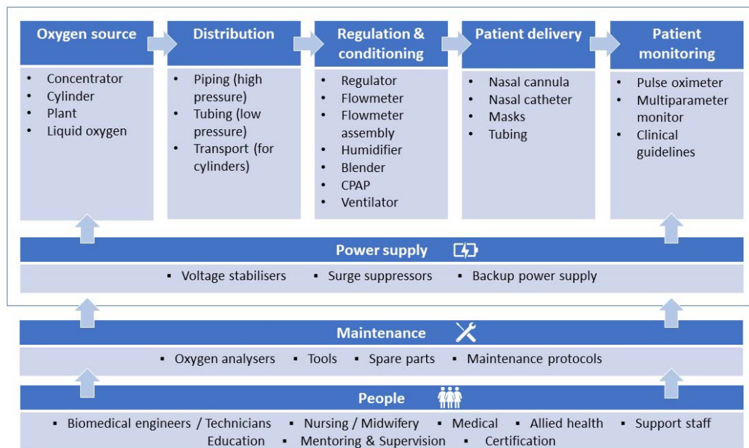
Figure 1 Hospital oxygen systems require a range of medical devices and other equipment and supplies (Adapted from WHO-UNICEF Technical Specifications and Guidance for Oxygen Therapy Devices)
