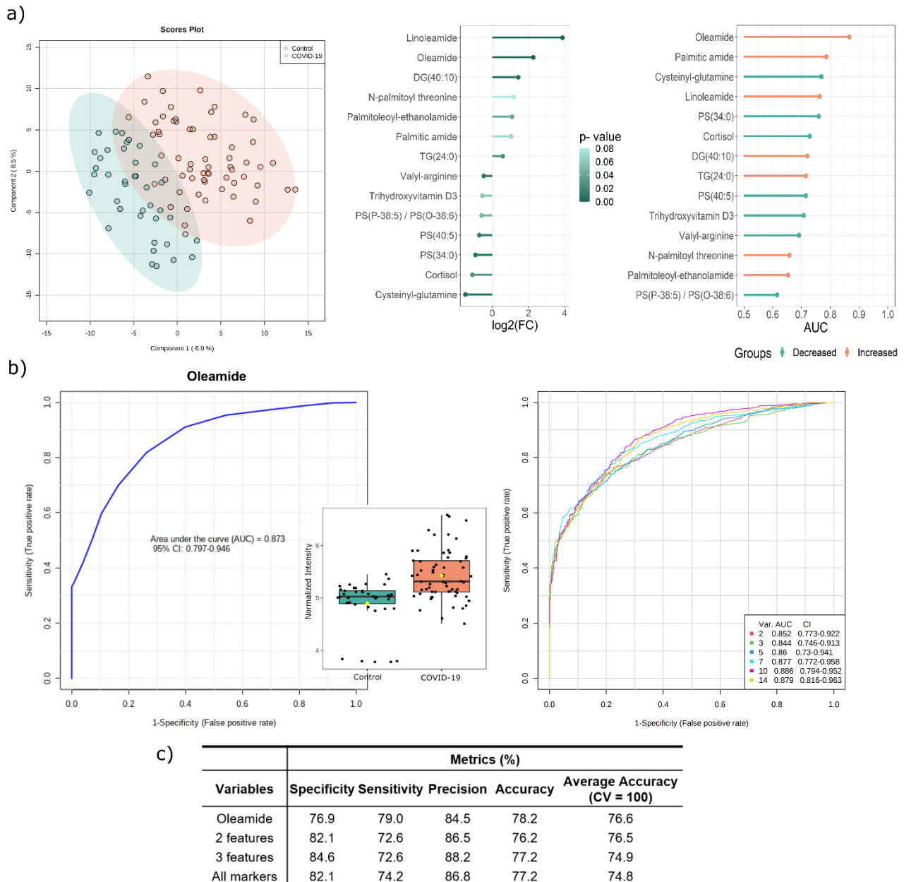
Figure 2. PLS-DA plot discriminated COVID-19 from Control group with listed annotated markers according to \log_2(\text{FC}) and p-value, and AUC (a). A ROC curve using Oleamide data, the most prominent marker ranked by AUC and a multivariate ROC curve was used to evaluate the influence of variable number (b) on model performance (c).
