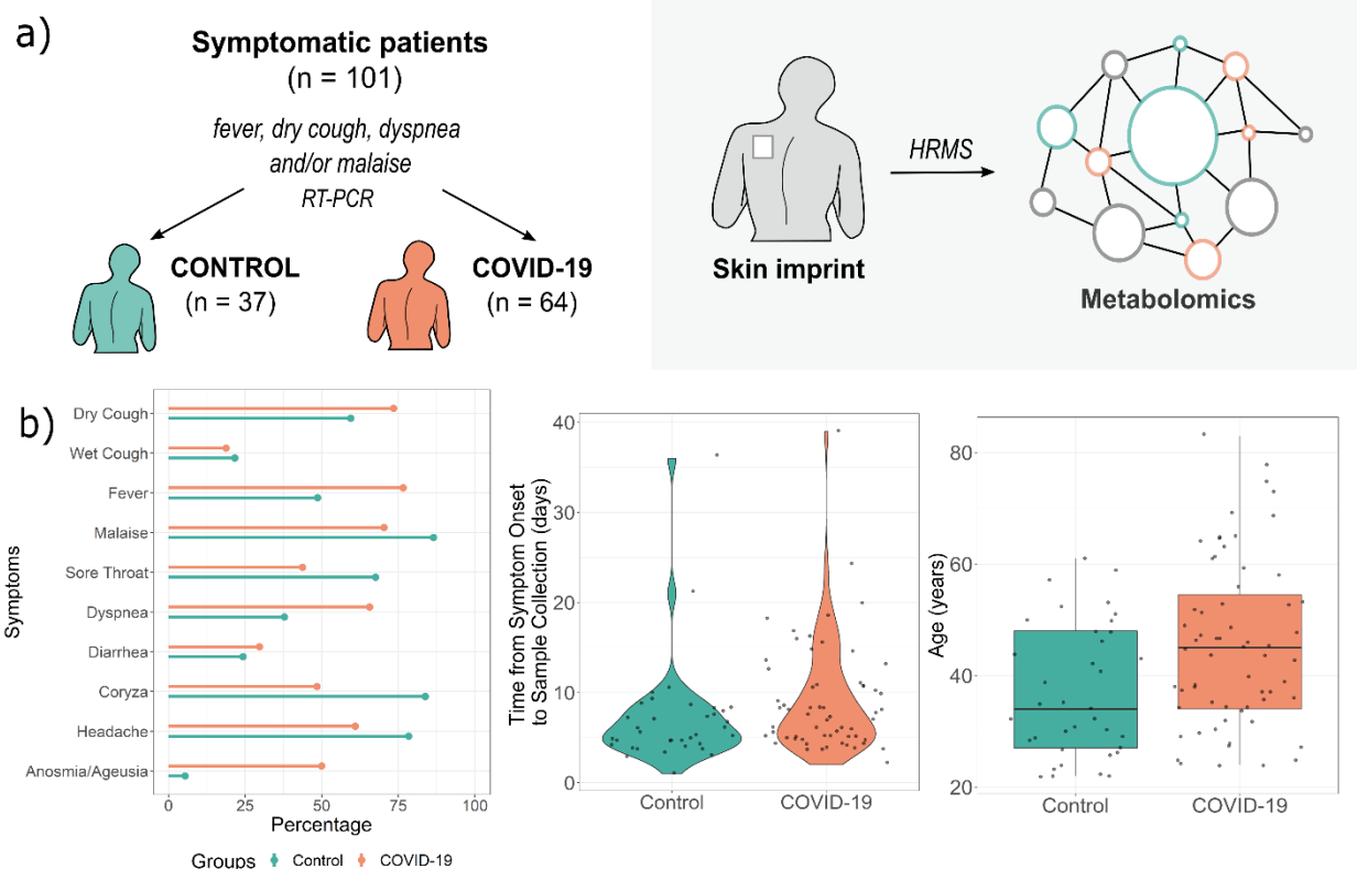
Figure 1. Study design (a) and patient symptoms distributions and age characteristics (b). HRMS – high-resolution mass spectrometry, RT-PCR – reverse transcriptase- polymerase chain reaction.
