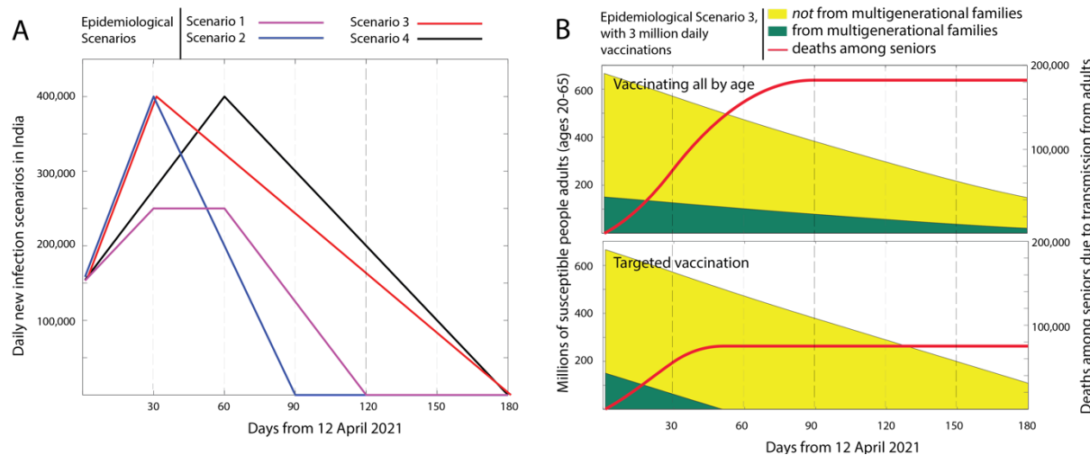
Figure 2. COVID-19 development scenarios and deaths avoided. A. The four COVID-19 development scenarios considered in this study. Scenario 1 is the most conservative scenario considering the daily infections on 12 April 2021. The peak of daily infections in all other scenarios is assumed to be 400,000 and is based on the average ratio of second to first peak observed in countries with the most infections ( Supplementary Table 1 ). B. Comparison of two strategies based on (top) no-selectivity in vaccinating members of multigenerational families and (bottom) preferential vaccination to younger members of multigenerational families for scenario 3. The deaths reduced among the Seniors by vaccinating the adults in all four scenarios is shown in Table 2 .
