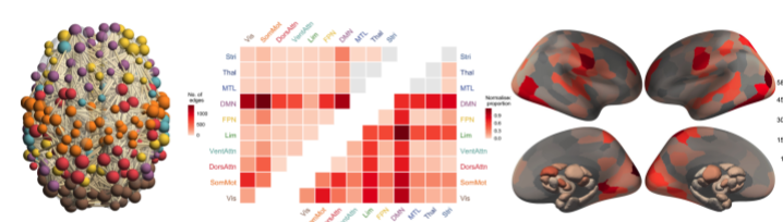
Figure 1 – Baseline and short-term longitudinal functional connectivity changes in antipsychotic-naïve patients. Legend shows the Schaefer network parcellation 29 and the Tian subcortex parcellation 30 (Scale II). Each of the four panels contains three figures (from left to right): (1) a visualisation of the significant NBS subnetwork, with the nodes coloured by network and weighted by degree; (2) a heatmap of the proportion of edges within the NBS component that fall within each of the canonical networks as represented quantified using raw (upper triangle) and normalized (lower triangle) proportions (see Supplement for details); and (3) surface renderings depicting the number of edges in the NBS subnetwork attached to each brain region. Vis, Visual network; SomMot, Somatomotor network; DorsAttn, Dorsal Attention network; VentAttn, Ventral Attention network; Lim, Limbic network; FPN, Frontoparietal network; DMN, Default mode network; MTL, medial temporal lobe (amygdala and hippocampus); Thal, Thalamus; Stri, Striatum. Subcortex: PUT, putamen; NAc, nucleus accumbens; CAU, caudate nucleus; GP, globus pallidus; HIP, hippocampus; AMY, amygdala; THA, thalamus; a, anterior; p, posterior; v, ventral; d, dorsal; m, medial; l, lateral; s, superior; i, inferior.
