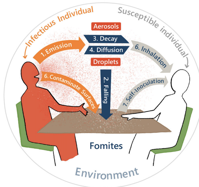
Fig 11. Schematic of processes in the epidemiological model.
