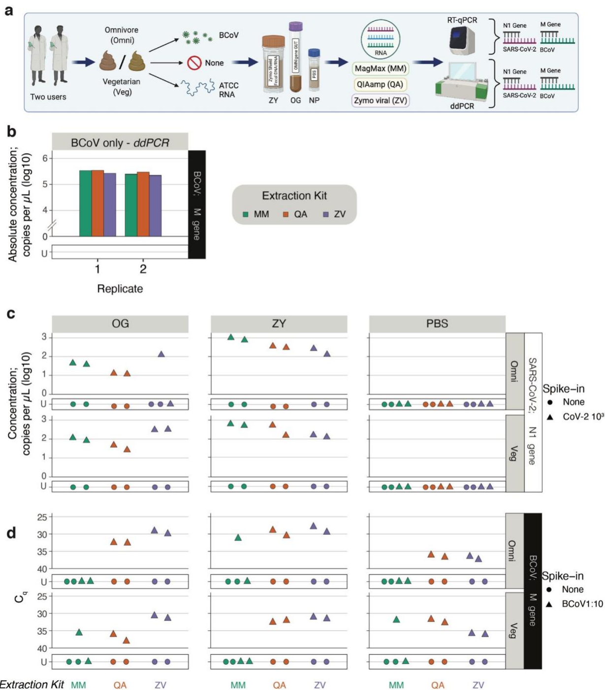
729 730 Supplementary Fig. 4 Performance of preservation and extraction of SARS-CoV-2 and BCoV RNA from 731 non-standardized stool samples from healthy donors. a. Two independent users performed this experiment. Stool 732 samples were collected from healthy omnivorous (Omni) and vegetarian (Veg) donors and spiked with ATCC CoV- 733 2 RNA or BCoV vaccine or equal volume of PBS (no RNA). Spiked stool was preserved in the OMNIgene-GUT kit 734 (OG), Zymo DNA/RNA shield buffer (ZY) and PBS. RNA was extracted from these samples using the MagMAX 735 Viral/Pathogen Kit (MM), QIAamp Viral RNA Mini Kit (QA) or Zymo Quick-RNA Viral Kit (ZY). RNA was 736 assayed using ddPCR and RT-qPCR targeting the SARS-CoV-2 N1 gene or BCoV M gene. b. As an extraction 737 control, RNA was isolated from the BCoV vaccine directly without the stool matrix using MM (green), QA (orange) 738 and ZY (purple) kits. Each user included a set of these extractions (indicated in the x-axis). Absolute concentration
