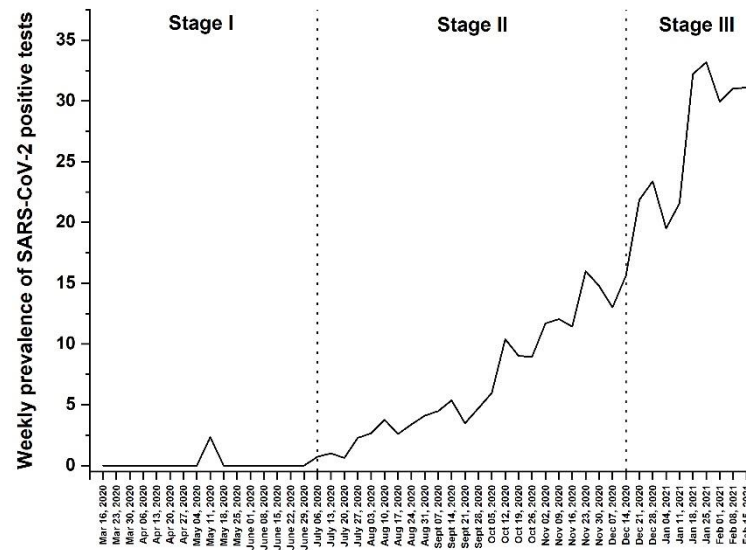
Figure 2: Weekly prevalence of SARS-CoV-2 positive cases between March 16, 2020 and February 21, 2021.
