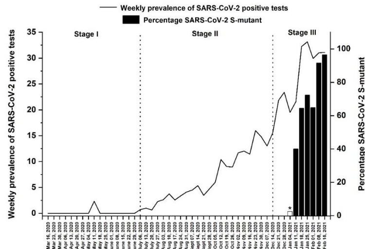
Figure 4: Weekly prevalence of SARS-CoV-2 positive tests and the percentage of S-mutant variant(s) among SARS-CoV-2 positive cases between March 16, 2020 and February 21, 2021.
