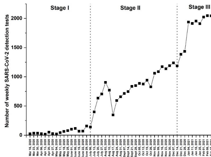
Figure 1: Number of weekly SARS-CoV-2 detection tests performed between March 16, 2020 and February 21, 2021.
