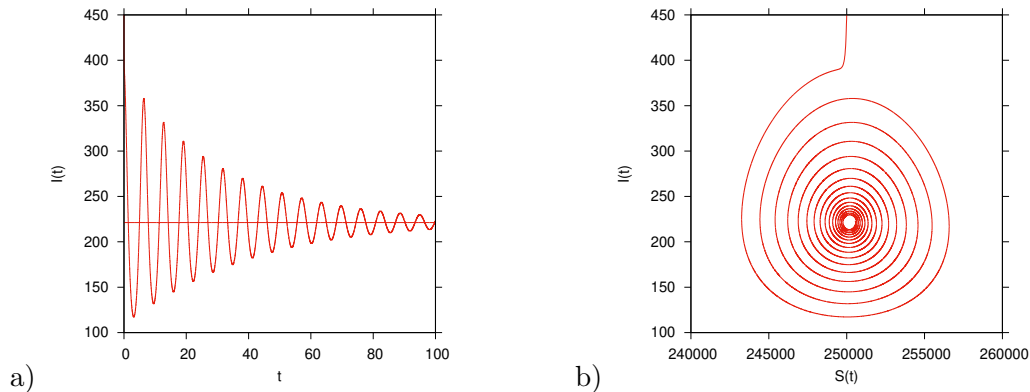
Figure 1: a) Time series of infected and b) state space plot of infected versus susceptibles in the SIRUV model with initial conditions close to the endemic fixed point. After an initial transient of decreasing infected I , oscillations symmetrically around the fixed point are observed.
