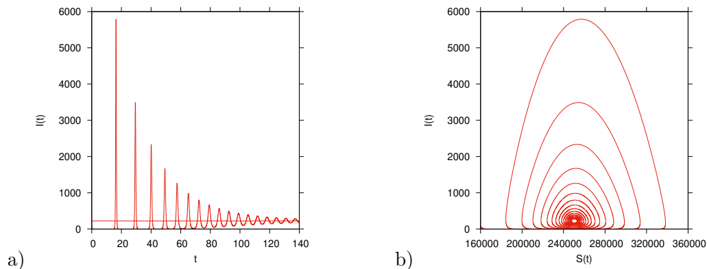
Figure 3: Time series of infected and state space plot of infected versus susceptibles in the SIRUV model. Initial conditions far away from the endemic fixed point, S_0 = 0.17 \cdot N , I_0 = 0.0001 \cdot N , and small number or no infected mosquitoes. After long times with low infection rate and slow build up of susceptibles we observe fast large outbreaks of infected, burning out large proportions of susceptibles (slow-fast regime). Then we observe a gradual transition to oscillations into the endemic fixed point with the known dynamics in the vicinity of the fixed point described (center manifold regime).
