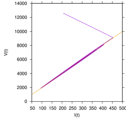
Figure 4: Quadratic approximation of z_3 = z_3(z_2, z_1) for continuously varying z_2 and z_1 = 0 in comparison with the trajectory spiralling into the fixed point. The quadratic expression gives essentially the linear relation between V and I again, namely V(I) = \frac{\vartheta}{\nu} \frac{M}{N} I(t) .
