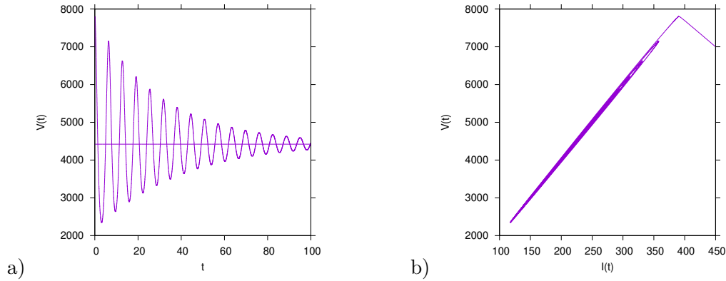
Figure 2: a) Time series of infected mosquitoes and b) state space plot of infected humans versus infected mosquitoes in the SIRUV model with initial conditions close to the endemic fixed point. The infected mosquitoes follow after a short transient period the infected humans with V(I) \approx \frac{\vartheta}{\nu} \cdot \frac{M}{N} \cdot I = 2 \cdot 10 \cdot I(t) .
