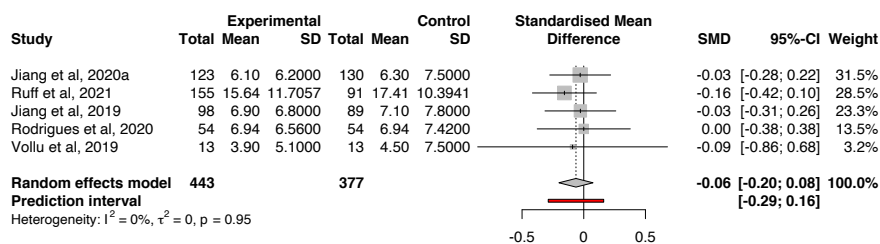
Figure 2: Random effects meta-analysis
