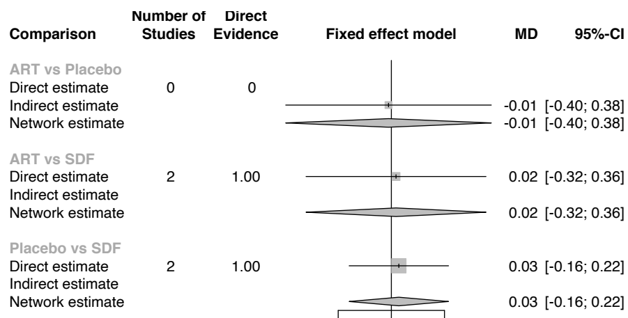
Figure 3: Subnetwork 1 forest plot, network meta-analysis
