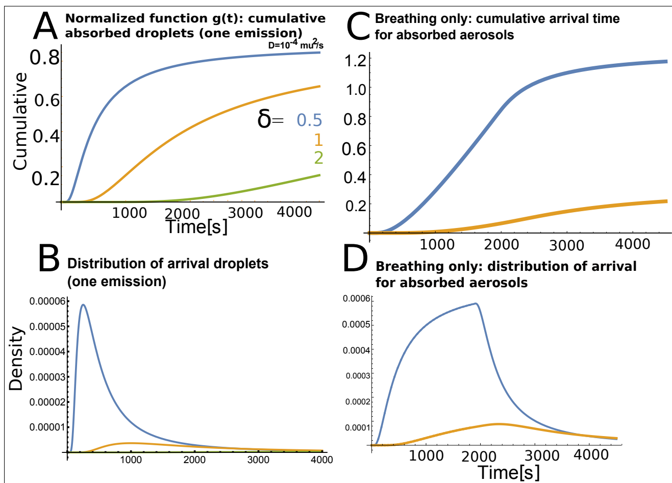
Figure S6: Cumulative and Distribution of viral particles arriving to a target person. Cumulative arrival (A) and distribution (B) of arrival for one event and rhythmic breathing, where 10 viral particles are emitted every minutes during 1800s, after the person leave the room.
