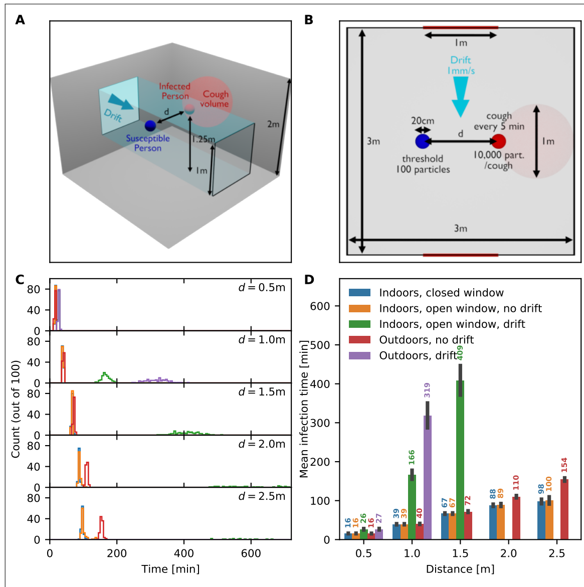
Figure 2: Infection times when an infected person is coughing once every 5 minutes. (A) 3D schematic representation of a closed room containing an infected (red) and a susceptible (blue) person separated by a variable distance d . The spherical volume in which 10^4 coughed particles are dispersed instantly is shaded red. As before, the room contains two windows which can be either open or closed with a possible drift between the windows. (B) Overhead view of (A). Room and window dimensions are displayed in the schematics. (C) Distribution of time of infection for distances d = 0.5, 1, 1.5, 2 and 2.5\text{m} and the following scenarios: Indoors with windows closed (blue), indoors with open windows, indoors with open windows and a drift, outdoors without drift (red), and outdoors with drift (purple). (D) Mean infection times for all scenarios. Missing bars indicate scenarios in which at least one realization had an infection time beyond 12 hours.
