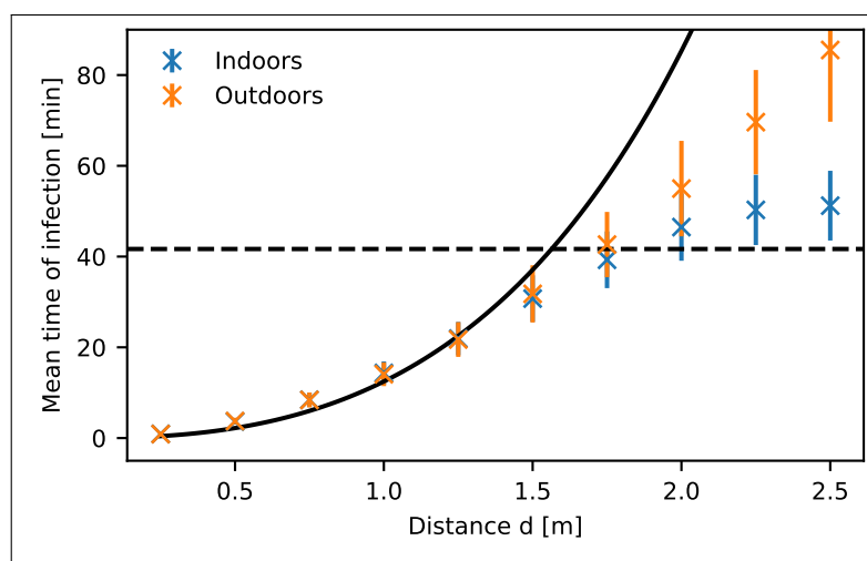
Figure S4: Mean infection time as a function of distance for a single cough The mean infection time as a function of distance d from simulations (crosses) for the indoor case with windows closed (blue) and the outdoor case without any drift (orange) when the infected person is coughing once. Error bars indicate the standard deviation. The solid line shows \tau_{inf} from equation 12, together with the crossover time \tau_c (dashed black line). Note that the threshold is set to 2 particles here.
