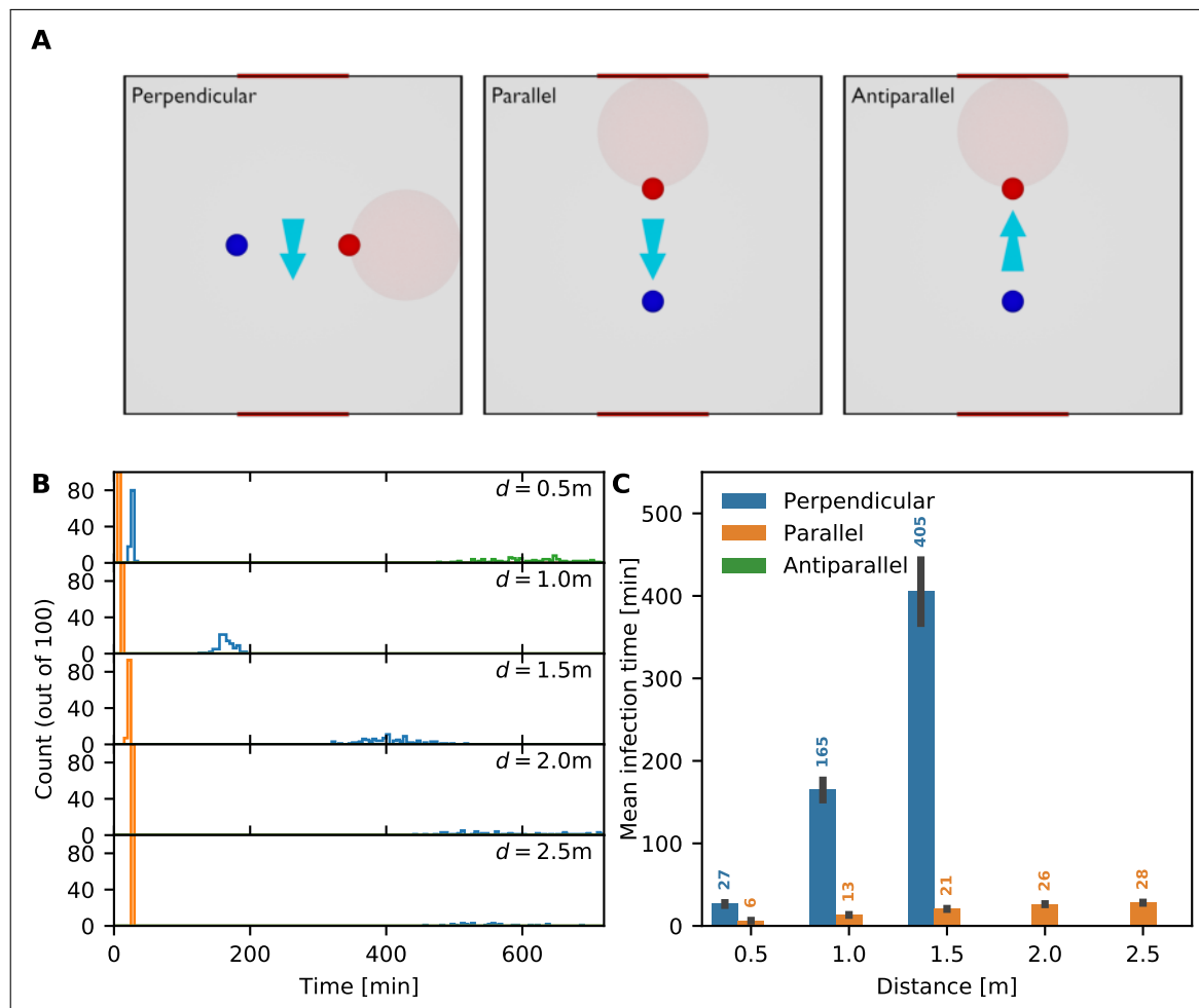
Figure S1: Influence of the direction of air movement. The mean time to infection as a function of distance and air movement direction for an infected person breathing in a room with open windows. (A) The light blue arrow indicates the direction of air movement / ventilation between the two windows. The direction of infection between the infected person (red circle) and the susceptible person (blue circle) can be perpendicular (left panel), parallel (middle panel) and antiparallel (right panel) to the direction of air movement. (B) Distribution of time to infection for distances d = 0.5, 1, 1.5, 2 and 2.5\text{m} and the scenarios: perpendicular (blue), parallel (orange) and antiparallel (green). (C) Mean infection time for the different scenarios. Missing bars indicate scenarios in which at least one realization had an infection time beyond 12 hours.
