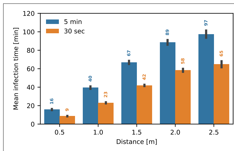
Figure S2: Influence of the cough interval. Mean time to infection for two different cough intervals, 5 minutes (blue) and 30 seconds (orange), and increasing distances d between the infected and susceptible persons. Error bars indicate the standard deviation.
