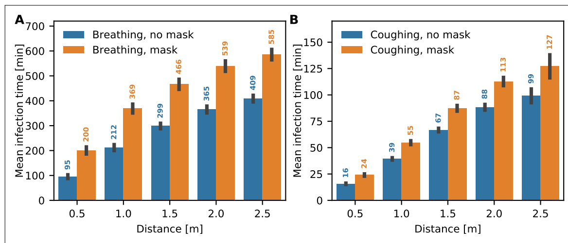
Figure 3: Effect of wearing a mask rejecting on average 2.8th particles for everyone accepted . (A) Mean infection times for various distances d = 0.5, 1, 1.5, 2 and 2.5\text{m} (indoors with windows closed), with and without mask when the infected person is breathing only. (B) Mean infection times for the same scenario as in (A), except that the infected person is coughing every 5 minutes.
