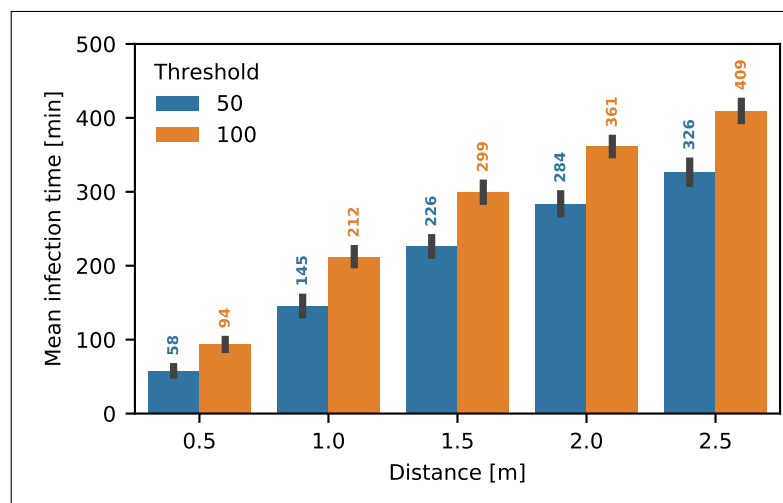
Figure S3: Influence of the threshold number of particles required for infection in the breathing case. Mean time to infection for two different values of the threshold, 50 (blue) and 100 absorbed particles. Error bars indicate the standard deviation.
