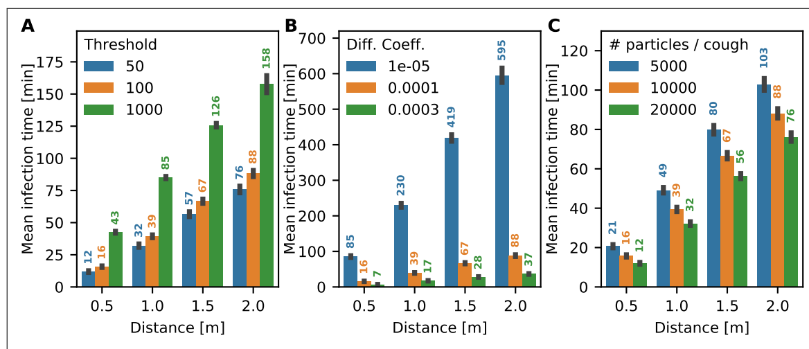
Figure 4: Sensitivity of the mean infection time to the threshold and diffusion coefficient . The mean infection time is estimated for an infected person coughing every 5 minutes in a room with windows closed. (A) Mean infection time for different values of the infection threshold count. (B) Influence of the diffusion coefficient. (C) Mean infection time vs the particle count contained in a cough.
