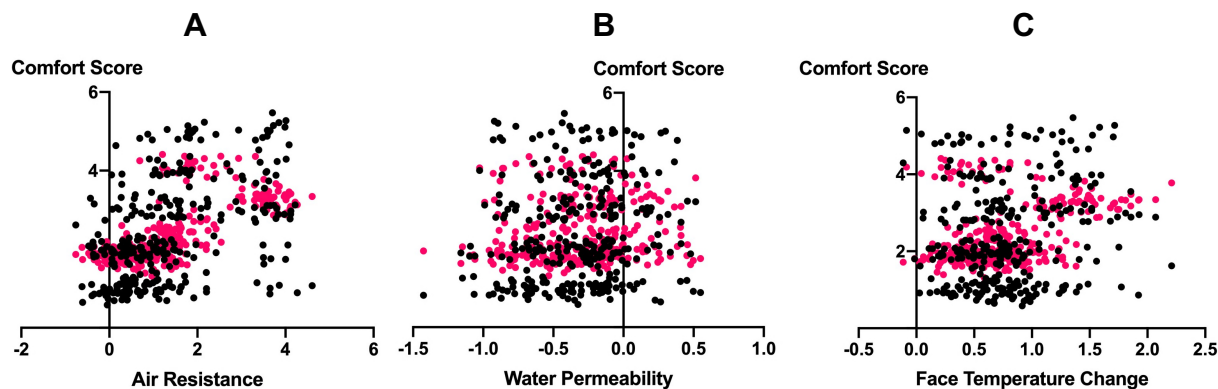
Figure 8: Comfort score, both actual scores (black) and scores predicted by the random forest machine learning model (pink), plotted against air resistance (A), water permeability (B), and face temperature change (C). These plots are shown with jittered values for ease of viewing. The random forest model creation and analysis was performed on original un-jittered data.
