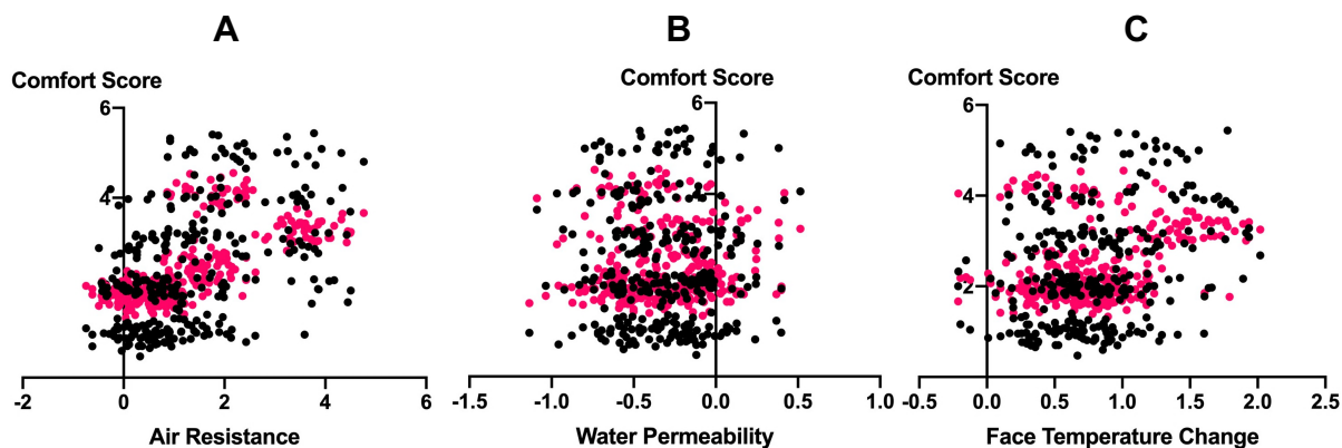
Figure 8: Comfort score, both actual scores (black) and scores predicted by the random forest machine learning model (pink), plotted against air resistance (A), water permeability (B), and face temperature change (C). These plots are shown with jittered values for ease of viewing. The random forest model creation and analysis was performed on original un-jittered data.
