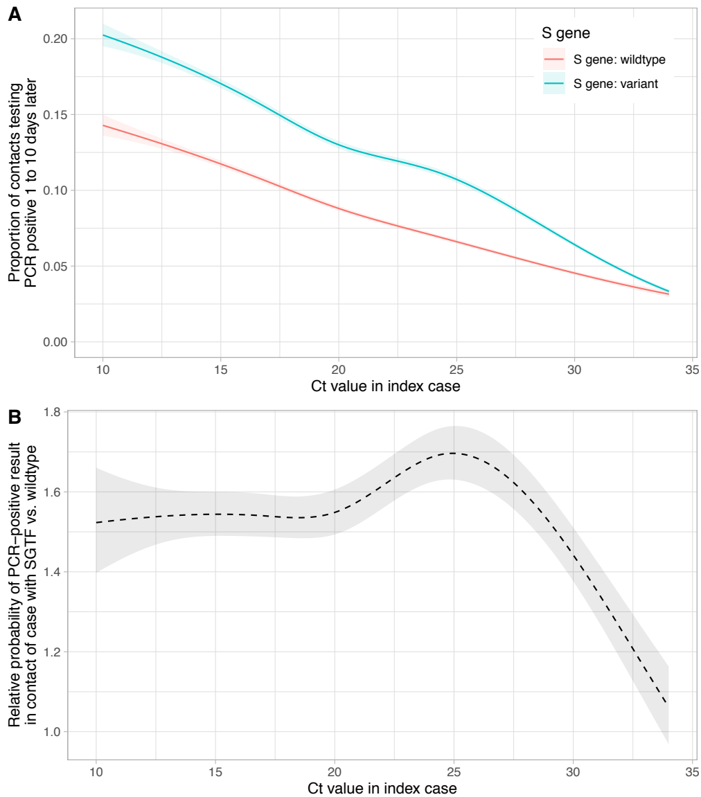
312 Figure 3. Relationship between PCR-positive results in contacts and index case Ct value and S gene 313 target failure (SGTF) indicative of B.1.1.7 variant. Panel A shows the proportion of contacts testing 314 by PCR-positive. Panel B displays the ratio of the two lines from panel A, i.e., the relative 315 infectiousness of index cases with SGTF vs. without SGTF. Model predictions are adjusted for index 316 case age, sex and ethnicity, contact index of multiple deprivation and incidence as in Figure 2.
