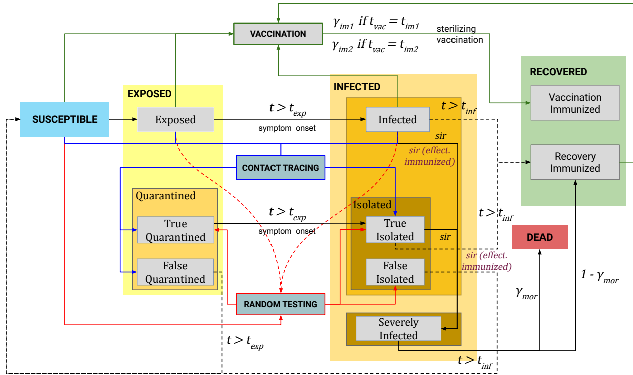
Fig. 1: The state chart of the particle-based SEIR epidemic simulator with effective and sterilizing vaccination.
