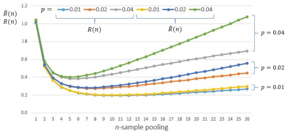
Fig. 3. Approximation of R(n; p) by \tilde{R}(n; p) ( R(n; p) \leq \tilde{R}(n; p) ) It becomes tighter as positive rate p becomes smaller, p = 0.04, 0.02, 0.01 .
