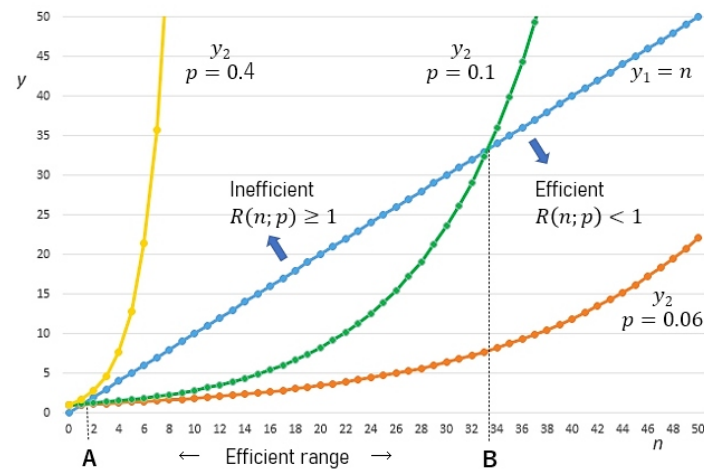
Fig. 2. Analysis of R(n; p) using functions y_1 = n and y_2 = (1 - p)^{-n}
