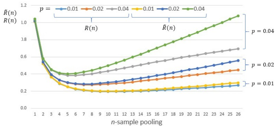
Fig. 3. Approximation of R(n; p) by \tilde{R}(n; p) ( R(n; p) \leq \tilde{R}(n; p) ) It becomes tighter as positive rate p becomes smaller, p = 0.04, 0.02, 0.01 .
