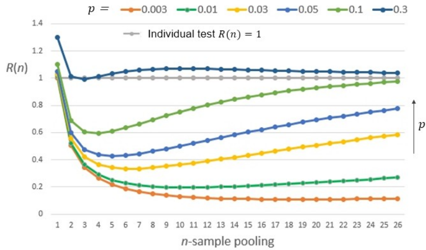
Fig. 1. Efficiency measure R(n; p) : “tests per samples” for pooling number n and positive rate p
