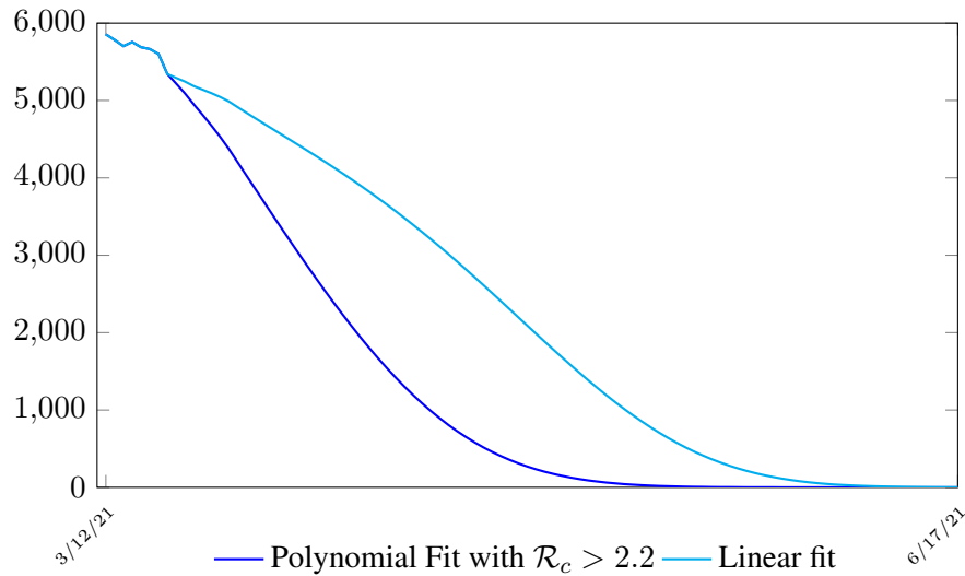
Figure 3.14: UK observed number of cases under 2 different \mathcal{R}_c(t) curve
