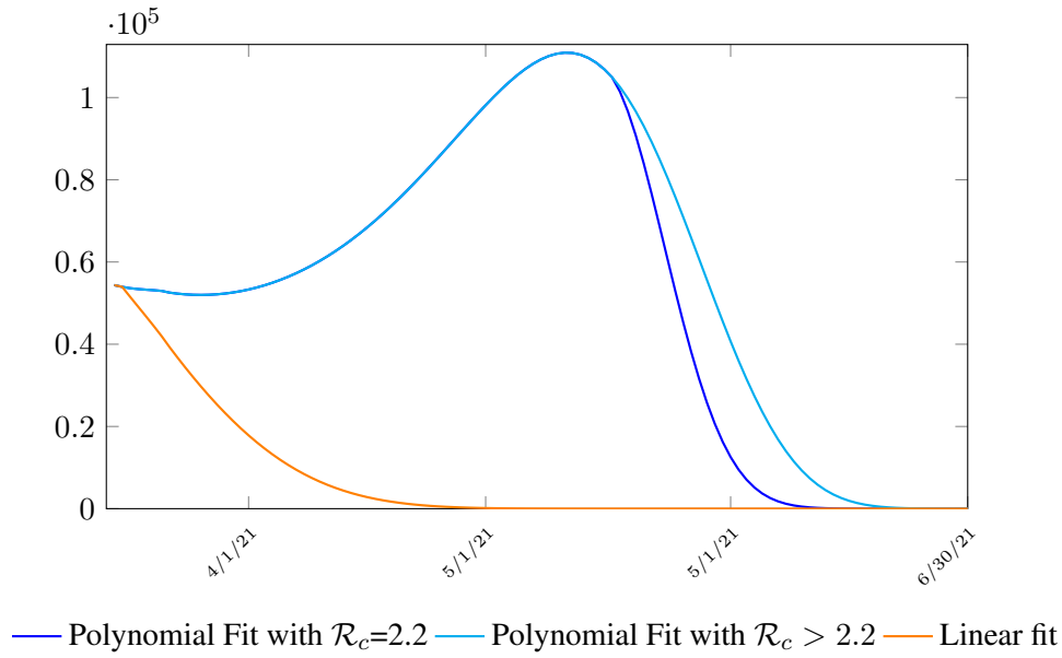
Figure 3.10: US observed number of cases under 3 different trajectories
