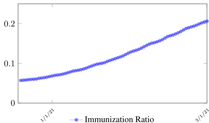
Figure 3.8: US effective immunization ratio
