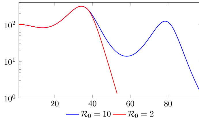
Figure 2.3: In this model simulation, 2 waves of infections is observed for \mathcal{R}_0 = 10 compared to only 1 for \mathcal{R}_0 = 2 (for \mathcal{R}_0 = 0 ) final daily infection number I_S^d(t) based on v_c(t) curves with R_0 = 2 and R_0 = 10
