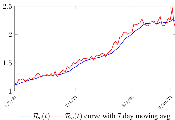
Figure 3.2: Israel's \mathcal{R}_c(t) curve
