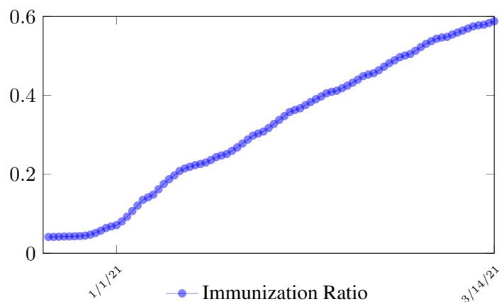
Figure 3.1: Israel effective immunization ratio
