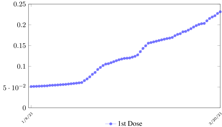
Figure 3.16: Serbia effective immunization ratio
