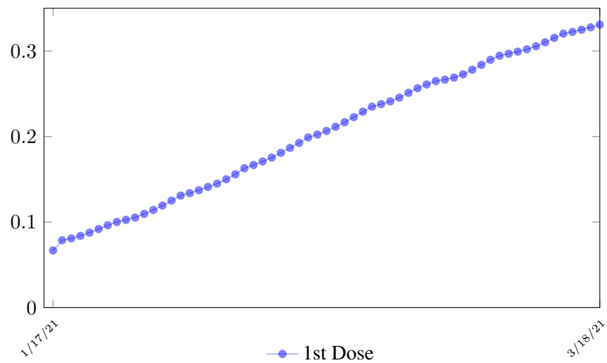
Figure 3.12: UK effective immunization ratio
