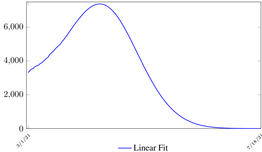
Figure 3.18: Serbia observed number of cases under \mathcal{R}_c(t) curve
