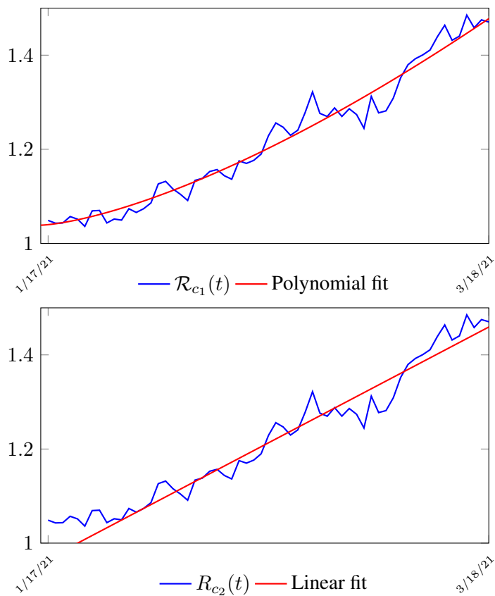
Figure 3.13: United Kingdom R_c(t) curve
