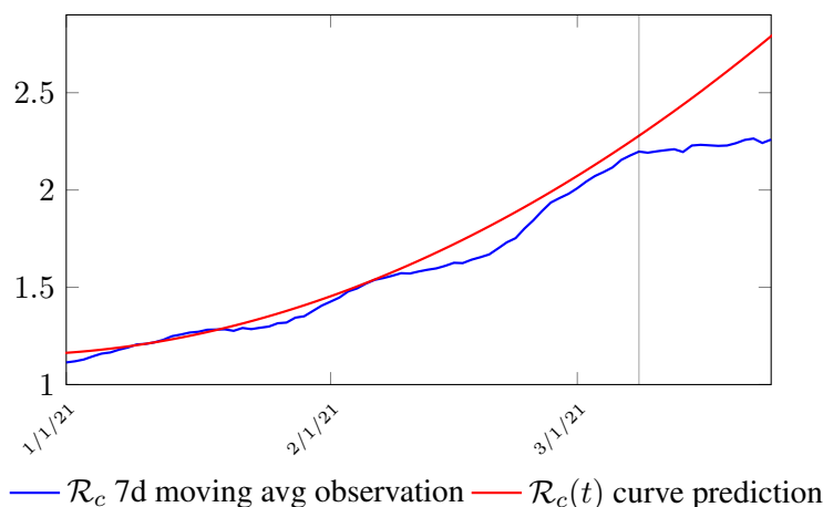
Figure 3.4: Observations starts to fall short from our \mathcal{R}_c(t) projection. Previous observations had also fall short from \mathcal{R}_c(t) projections, however, the gap has been much smaller, furthermore, the moving average was still increasing and not as a plateau as we observed now. The plateau starts at 3/8/21 indicated by the gray vertical divider.
