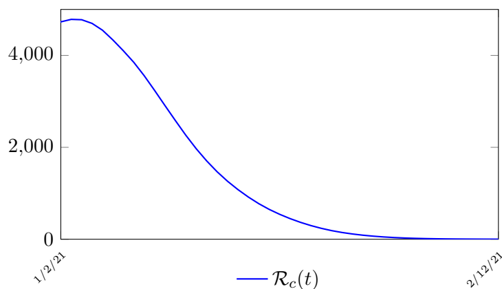
Figure 3.3: Israel's predicted daily infection if control \mathcal{R}_c = 1.1521 remained.
