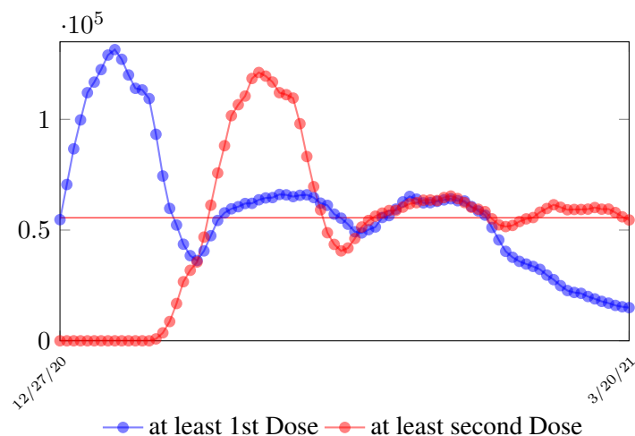
Figure 3.5: The observed Israel daily vaccination dosage administered for single and double doses during Feb 2021
