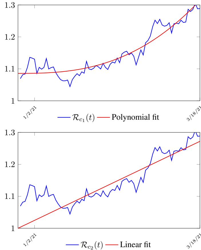
Figure 3.9: United States \mathcal{R}_c(t) curve
