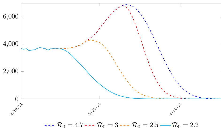
Figure 3.6: Israel predictions, left to right: \mathcal{R}_0 = 2.2 , \mathcal{R}_0 = 2.5 , \mathcal{R}_0 = 3.0 , and \mathcal{R}_0 = 4.7 . Its most likely that \mathcal{R}_0 = 2.2 . Other trajectories given higher possible \mathcal{R}_0 is also shown. Notice that even for \mathcal{R}_0 = 2.2 trajectory is somewhat higher than the actual number of infection observed. This is reasonable since the curve is based on 7 day moving average.
