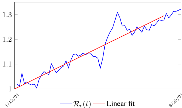
Figure 3.17: Serbia \mathcal{R}_c(t) curve
