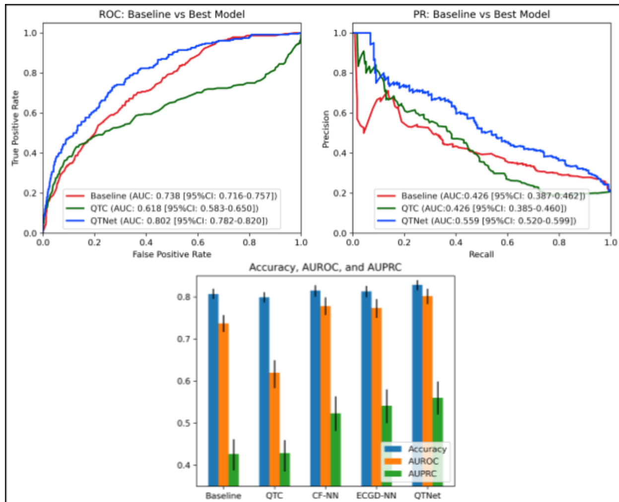
Figure. Performance of QTNet predicting diQTP. Compared models include the Baseline CF logistic regression model (Baseline), Reference QTc (QTC), NN trained on clinical features (CF-NN) and NN trained on ECG data (ECGD-NN). diQTP, drug induced QT prolongation; CF, clinical risk factors; NN, neural network.
