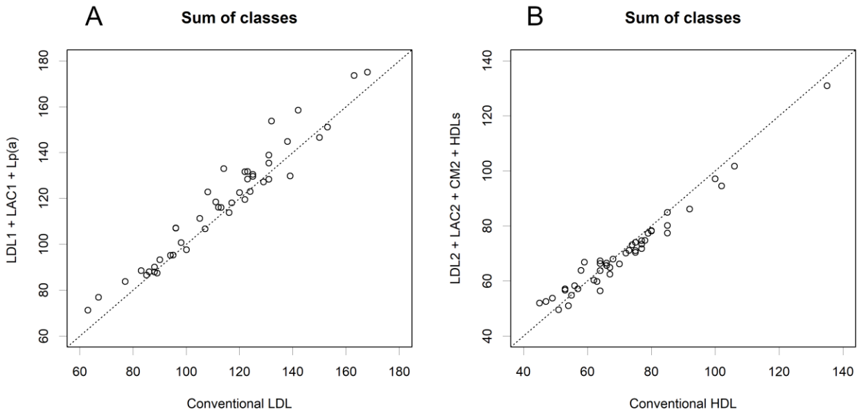
Fig. 4 Estimation of the sets of classes that are measured by a conventional method. If the conventional methods extract most of the cholesterol from particular classes, these would present the sum of the quantities of the classes. The combinations presented here were the ones with the highest correlation and the closest amounts.
