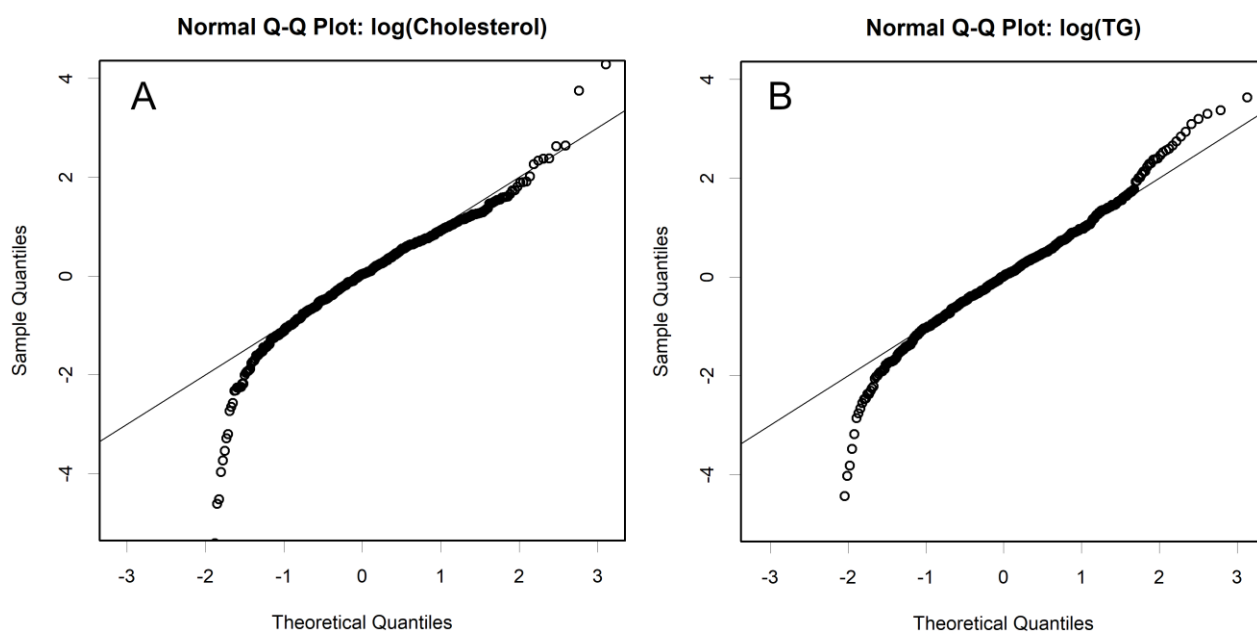
257 Fig. 3 Normal Q-Q plot of the logarithms of normalized data. Cholesterol (A.) and TG (B). Quantiles are 258 compared between the theoretical normal distribution and the z-normalized log-data. Here a lognormal 259 distribution will form a straight relationship.
