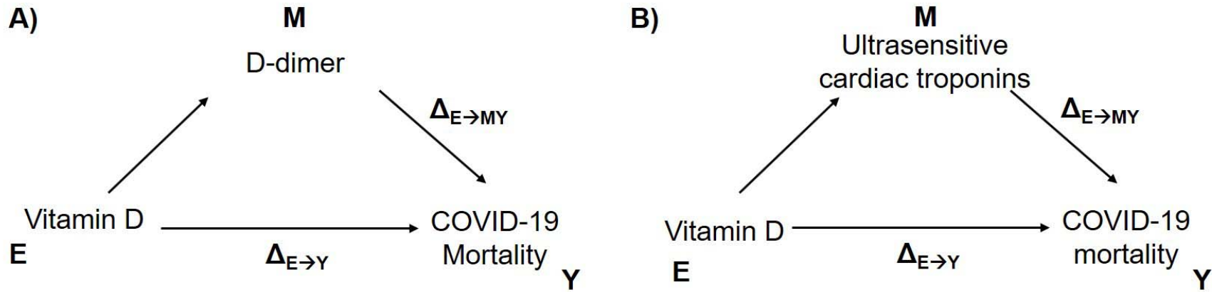
499 Figure 3. Model-based causal mediation analyses to investigate the role of Vitamin D on COVID-19 mortality mediated by D-dimer
