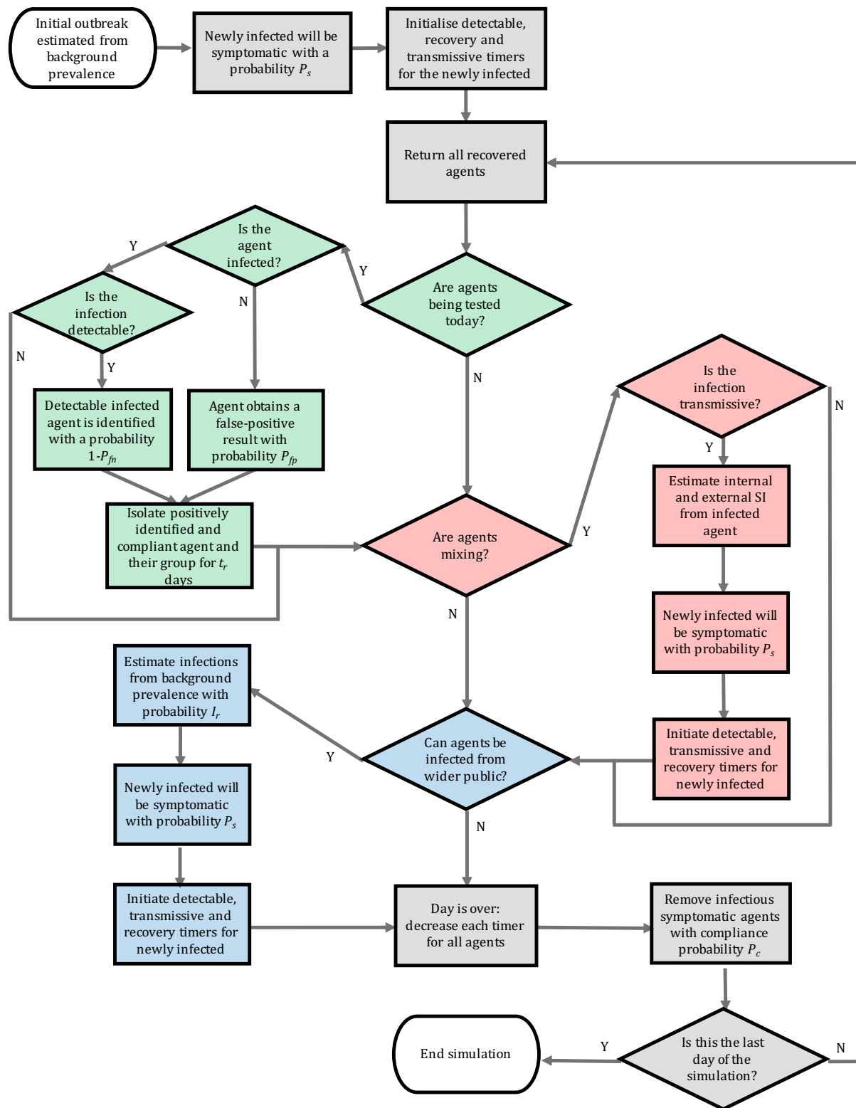
Figure 6: Flowchart illustrating the algorithm developed for the individual based model of infection spread. We highlight various subroutines using colours: grey is base infection routines, green is testing, red is secondary infection estimation and blue represents infections from outside the population. SI corresponds to secondary infections.
