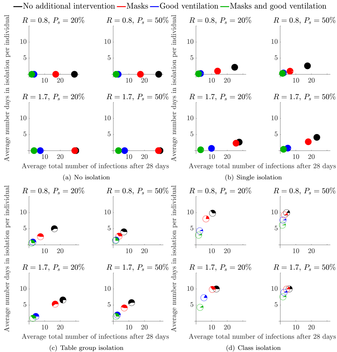
Figure 2: Mean number of infected students and average number of days absent per individual when no testing is employed, over a variety of isolation strategies and interventions in a secondary school environment. Each symbol represents a different intervention, see legend at the top of the figure for details and see Section 2.1 for a description of how each intervention influences the parameter values. Note that the 4 pie charts in (b) have visually small sectors representing isolation of healthy individuals with a false-positive test result.
