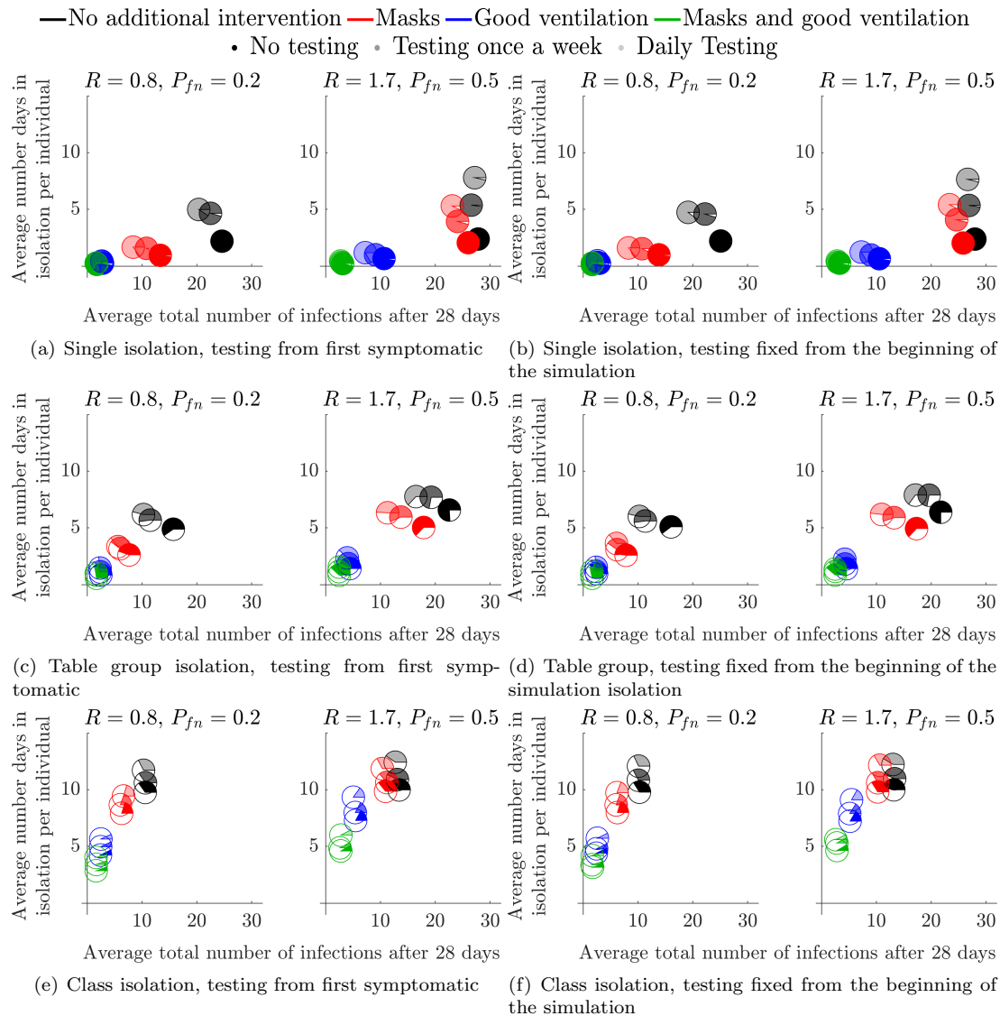
Figure 3: Mean number of infected students and average number of days absent per individual when testing is employed, over a variety of isolation strategies and interventions in a secondary school environment. Each symbol represents a different intervention, see legend at the top of the figure for details and see Section 2.1 for a description of how each intervention influences the parameter values.
