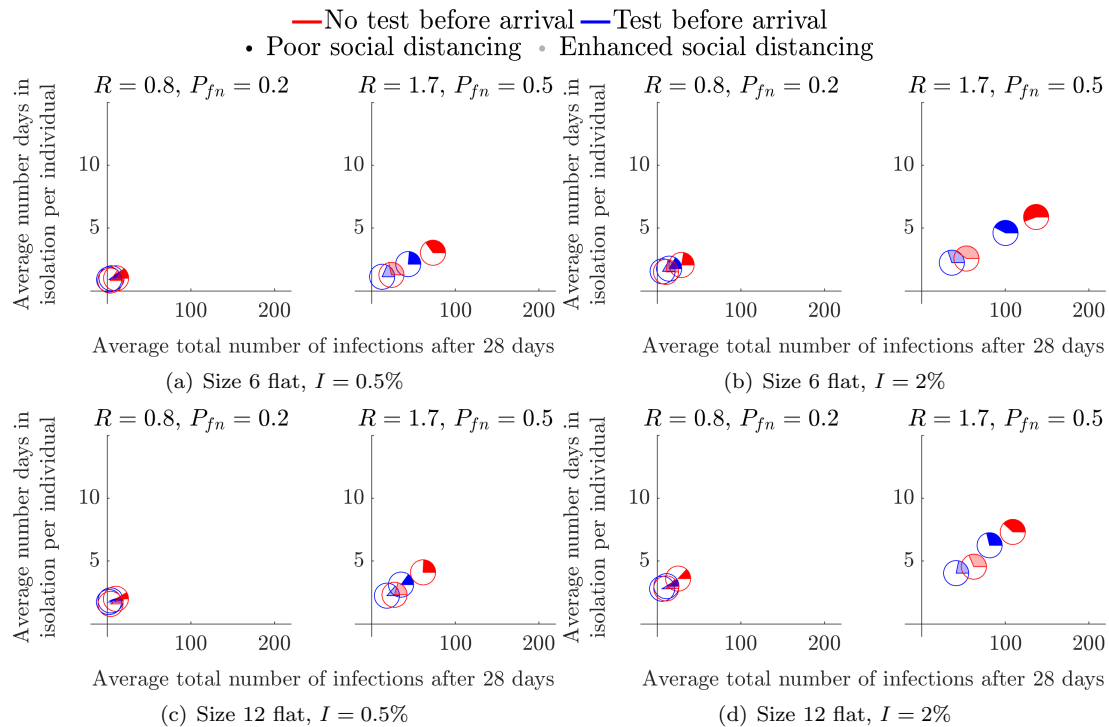
Figure 4: Considering the effects of a pre-term LFD test across flats of different occupancy (noted below each subfigure).
