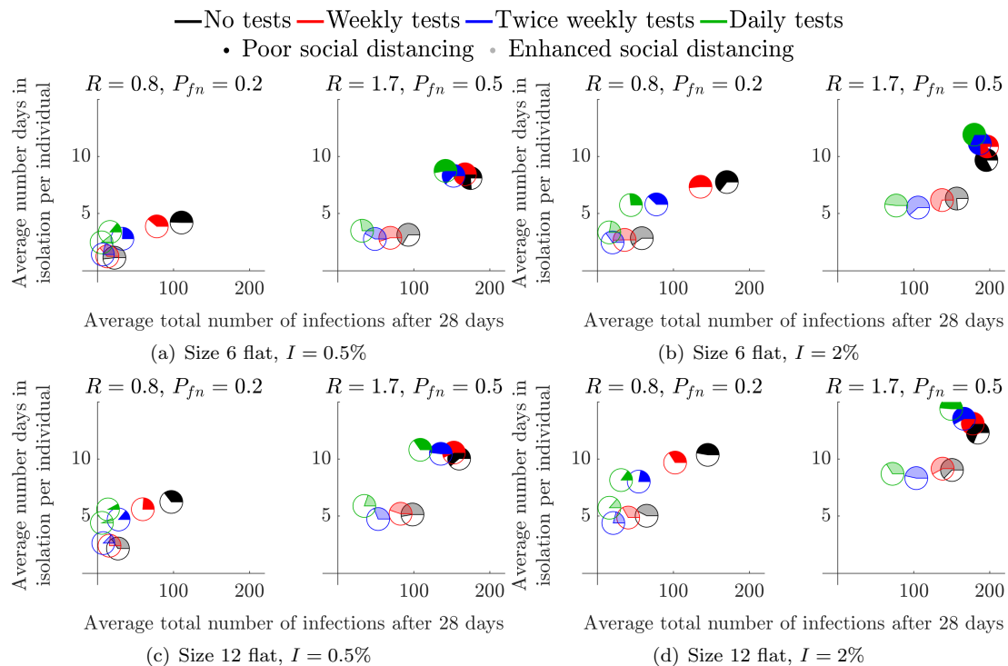
Figure 5: Considering the effects of a mid-term LFD test across flats of different occupancy (noted below each subfigure).
