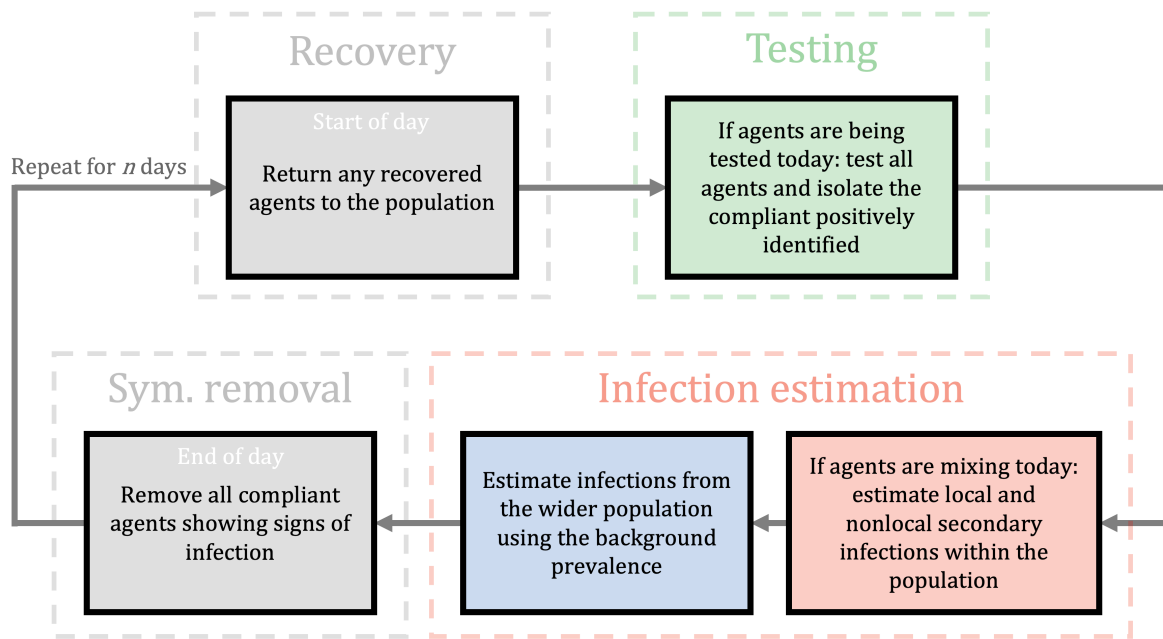
Figure 1: A flowchart illustrating the general iterative process controlling the dynamics of the discrete population over a typical day post simulation initialisation. Grey boxes represent actions that occur every day whereas the coloured boxes can be independently active/ inactive on any prescribed day. A single cycle accounts for a single day. We start each day at the recovery box which returns any isolating agents that have completed their isolation period. If testing is active, the individuals are tested using LFD, agents with a positive test are removed from the population for t_r days. If agents are allowed to mix, then we estimate secondary infections using R with context specific scalings ( e.g. NPIs). Next, if external infection sources are being considered, we estimate the number of infections to the susceptible population using the background prevalence. Finally, we remove any compliant symptomatic individuals that display the infection at the end of every day. For a detailed flowchart of the infection algorithm, see Appendix A.
