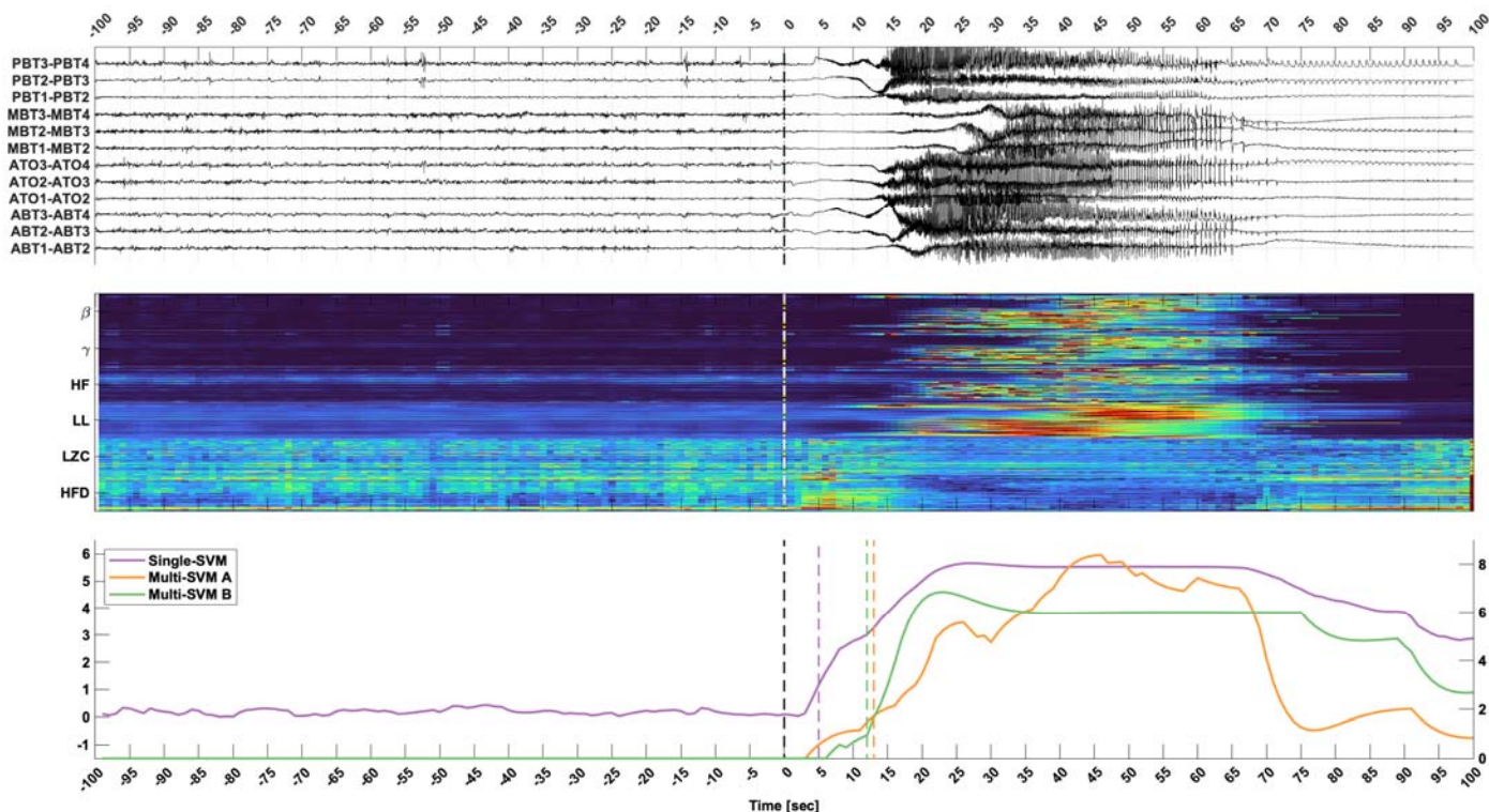
Figure 2. Early-onset detection. Top panel shows 200 seconds of the EEG of a selected number of channels where the seizure onset zone is localized. Middle panel shows the extracted features from the EEG. Bottom panel shows the postprocessed output for the different SVM configurations. The purple trace represents the single-SVM, the orange trace the multi-SVM A, and in green the multi-SVM B configuration, respectively. Dashed colored lines show when the event was detected for each SVM configuration. The dashed black line at time zero denotes the seizure onset as marked by the clinicians.
