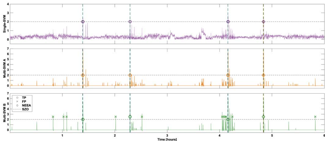
Figure 6. Long SVM output traces showing six-hour traces of the SVM output for all three configurations, single-SVM (purple), Multi-SVM A (orange), and Multi-SVM B (green). Seizure-onset markings are shown in vertical dashed black lines. Detection thresholds in horizontal dashed lines. TP detections are marked with a circle, FP are marked with a cross, and NEEA detections are marked with a diamond.
