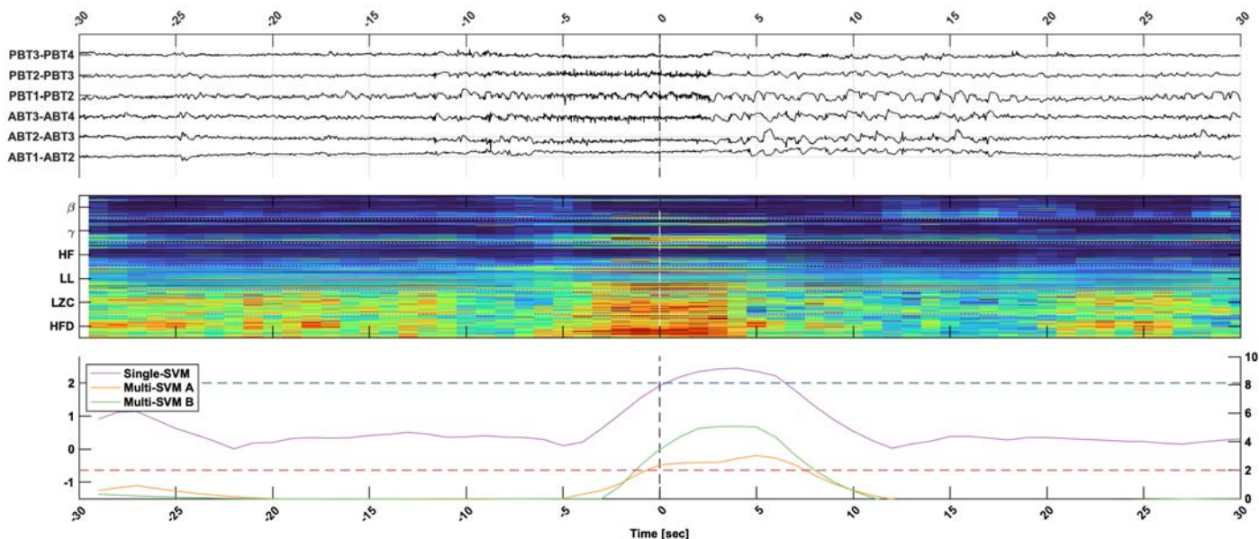
Figure 5. NEEA detection. Top panel, shows one minute of EEG trace, for subset of channels that show epileptiform activity. Middle panel, shows extracted features from the EEG. Bottom panel as in Figure 2 and 3 shows the postprocessed output of the different SVM configurations. Horizontal dashed lines show the detection threshold for the SVM configurations. In blue the threshold for the single-SVM and in red the threshold for the multi-SVM configurations. The dashed black line at time zero denotes the NEEA event marked by the clinicians.
