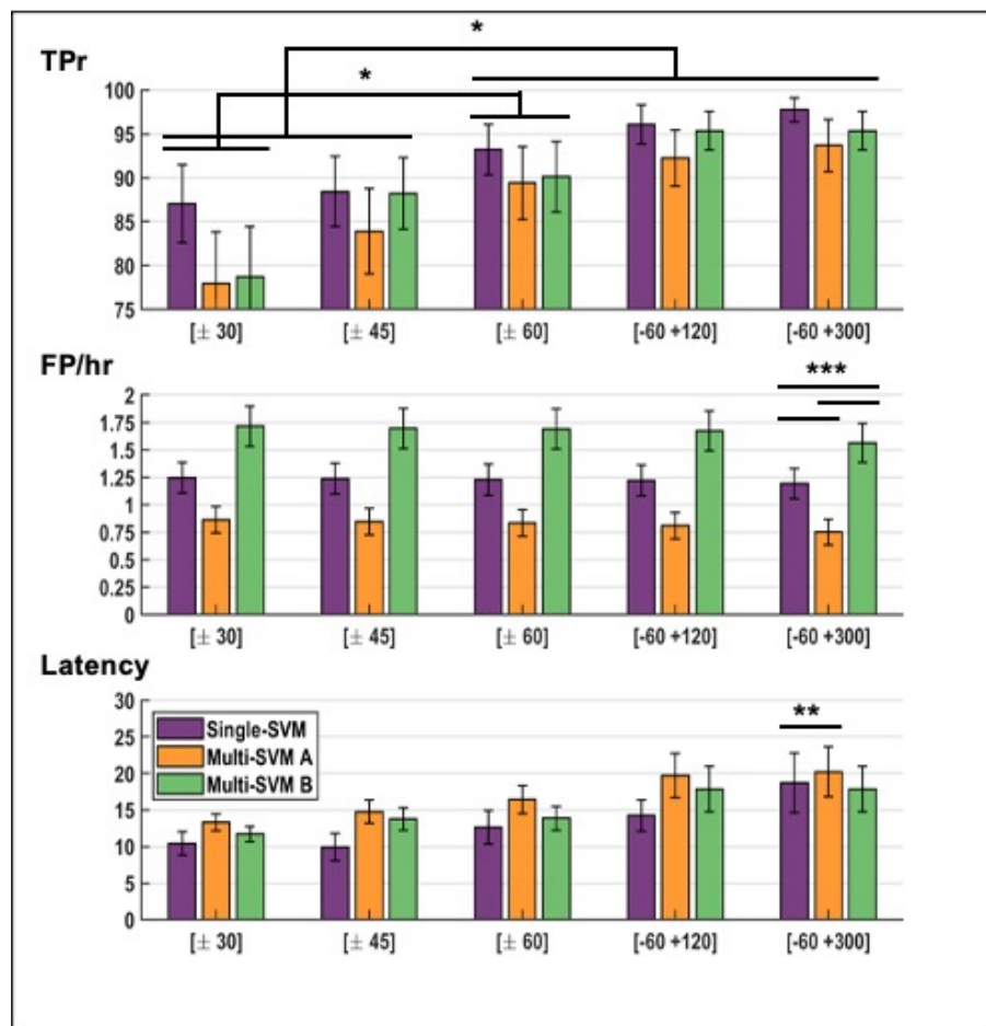
Figure 4. Results Stats in bar plots. The results are shown for TPr, FP/hr and Latency for the different SVM configurations as well as for the different detection window sizes. Statistical significance is shown for post-hoc analysis using Dunn's test (* p \leq 0.05 , ** p \leq 0.001 , and *** p < 0.0001 ).
