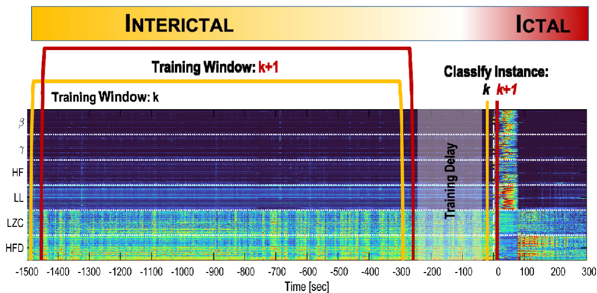
Figure 1. Dynamic training paradigm. Heatmap shows the extracted features from the EEG over time. Every second, a shifting 20-minute window of features is used for SVM training. This training window is delayed five minutes from the current instance to exclude any preictal data that might mislead the SVM in classification of the current instance.
