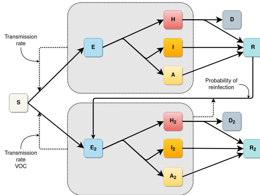
Figure 1: Diagram of the SEAIHRD model. S: Susceptible, E: Exposed (pre-symptomatic), H: Hospitalized (severe infected individuals), I: Infected (symptomatic individuals, not hospitalized), A: Asymptomatic. D: Deceased, R: Recovered. All the compartments are subdivided into 3 age classes, not represented here for simplicity. Compartments with no subindex are related to the wild variant, compartments with subindex 2 are related to the VOC P.1. Continuous lines represent flux between each compartment. Dashed lines represent infection pathways. Three parameters fitted by the model are indicated by the small arrows.
