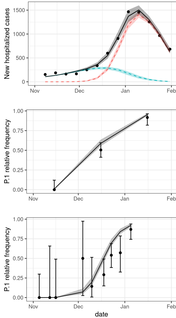
Figure 2: First panel: Weekly new hospitalized COVID-19 cases in Manaus city. Grey line represents the fitted values of total cases (all variants) by maximum likelihood estimation (MLE) of the parameters. Red (blue) line represents the fitted values of cases due to P.1 (wild) variant, black dots are nowcasted observed data of hospitalization. Second and third panels show the fittings to the P.1 time-series frequency of P.1 on datasets provided by (7) and (3) respectively. The area around the lines indicate the 95% CI of the expected values. The fitted values of the model parameters are presented in the first part of Table 1.
