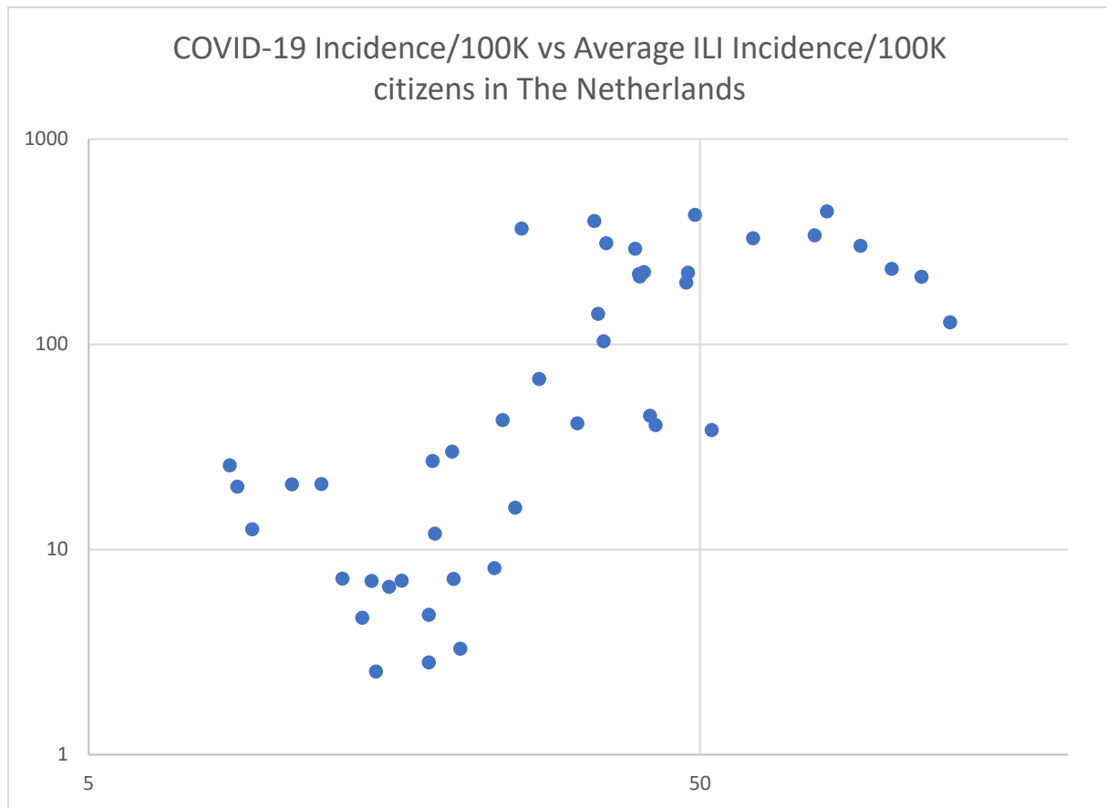
291 Fig. 2. Scatter diagram showing the relation between COVID-19 incidence/100K citizens (Y-axis) and the 292 seasonal, average ILI incidence/100K citizens (X-axis) in the Netherlands of the preceding 4 years.
