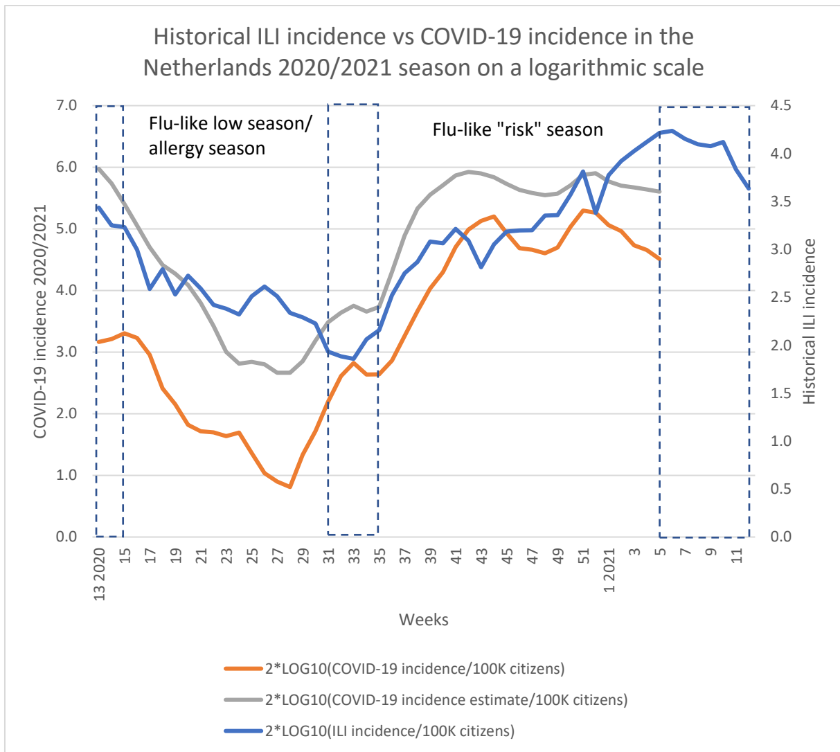
306 Fig. 2. Historical ILI incidence versus COVID-19 incidence per 100K citizens on the 1 to 10 logarithmic scale. It 307 visualizes how similar the COVID-19 time series based on hospitalizations is with the historic ILI time series.
