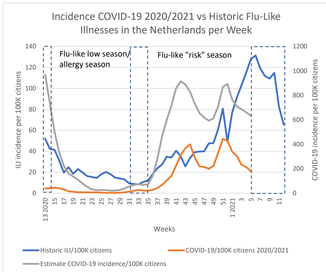
300 Fig. 1. Historical ILI incidence versus COVID-19 incidence per 100K citizens during the 2020/2021 season. 301 Peaks are all during flu season, and lows during the opposite season. The shaded periods are the typical period 302 in which seasonal switching occurs.
