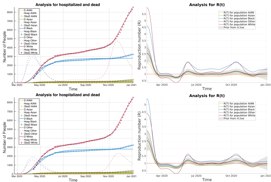
FIGURE 25. Analysis results when using peicwise updates to R(t) for MI. Top row: R^A with entries of all ones. Bottom Row: R^A for FLCs and NFLCs.
