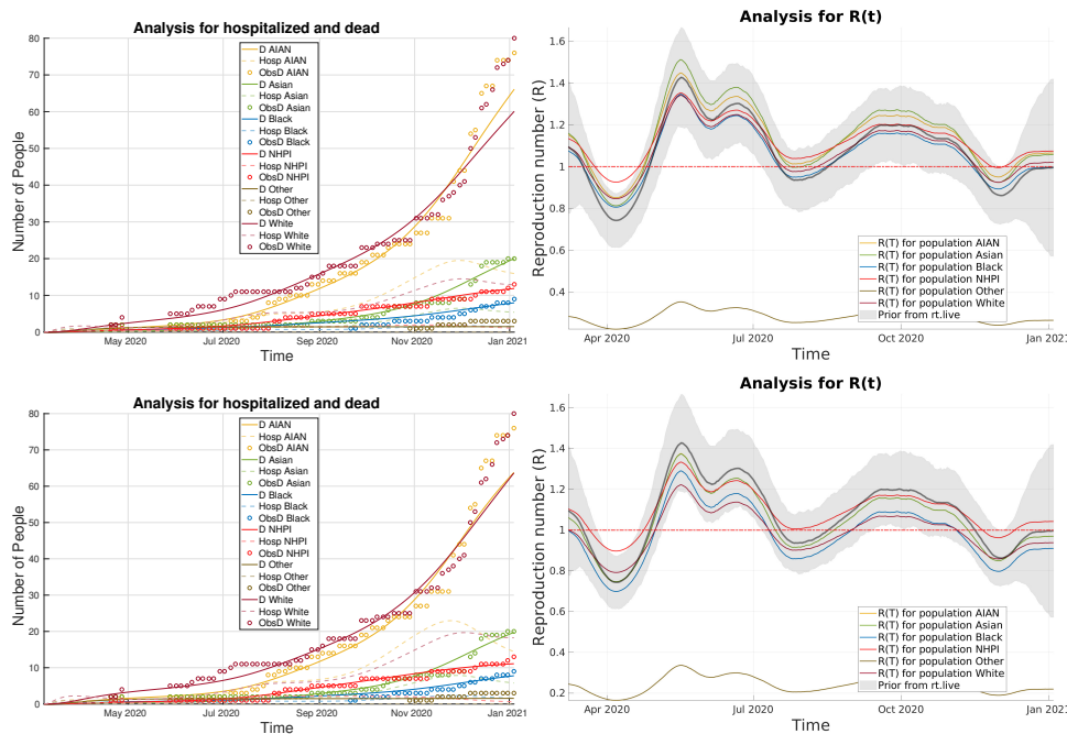
FIGURE 18. Analysis results when using peicewise updates to R(t) for AK. Top row: R^A with entries of all ones. Bottom Row: R^A for FLCs and NFLCs.
