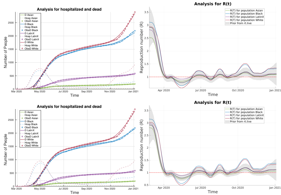
FIGURE 24. Analysis results when using peicewise updates to R_t(t) for MD. Top row: R^A with entries of all ones. Bottom Row: R^A for FLCs and NFLCs.
