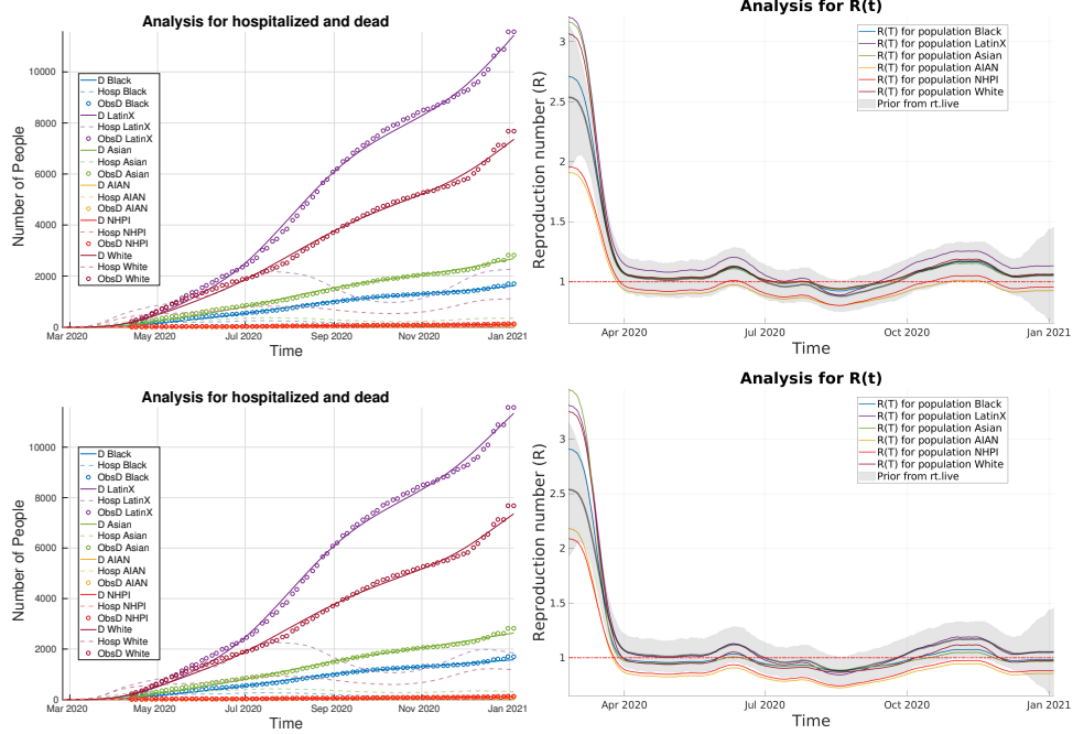
FIGURE 19. Analysis results when using peicwise updates to R(t) for CA. Top row: R^A with entries of all ones. Bottom Row: R^A for FLCs and NFLCs.
