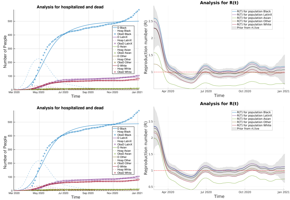
FIGURE 22. Analysis results when using peicwise updates to R(t) for DC. Top row: R^A with entries of all ones. Bottom Row: R^A for FLCs and NFLCs.
