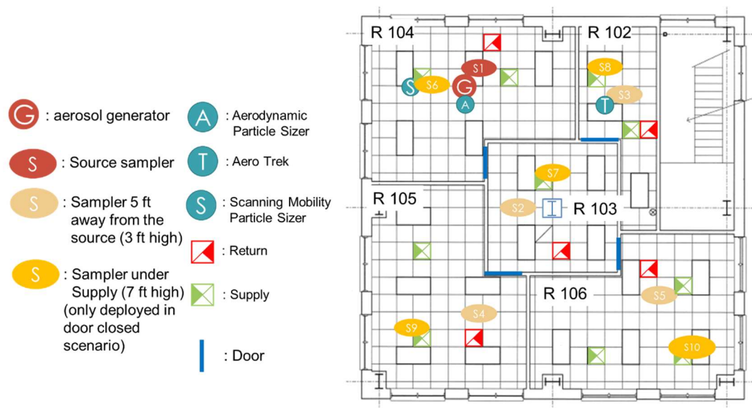
Figure 4. Location of samplers in the far-field campaign
