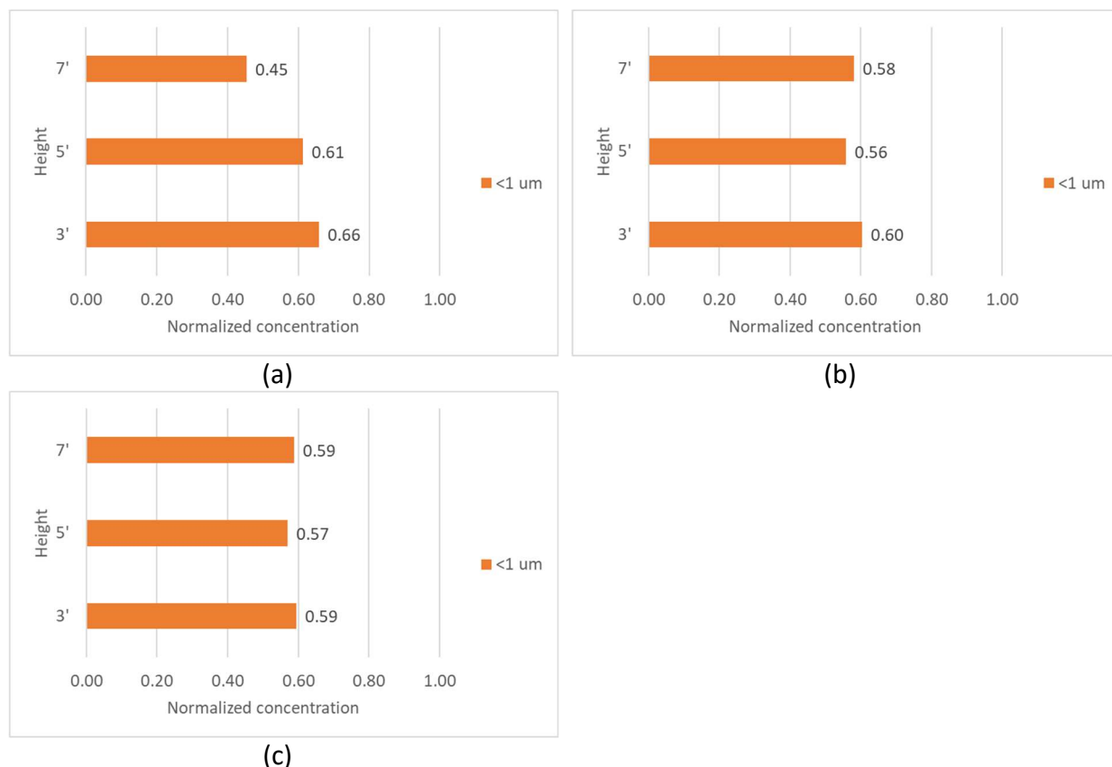
Figure 7. The spatial distribution of normalized concentration measured at (a) 6 ft, (b) 8 ft, and (c) 10 ft away from the source in the horizontal direction.
