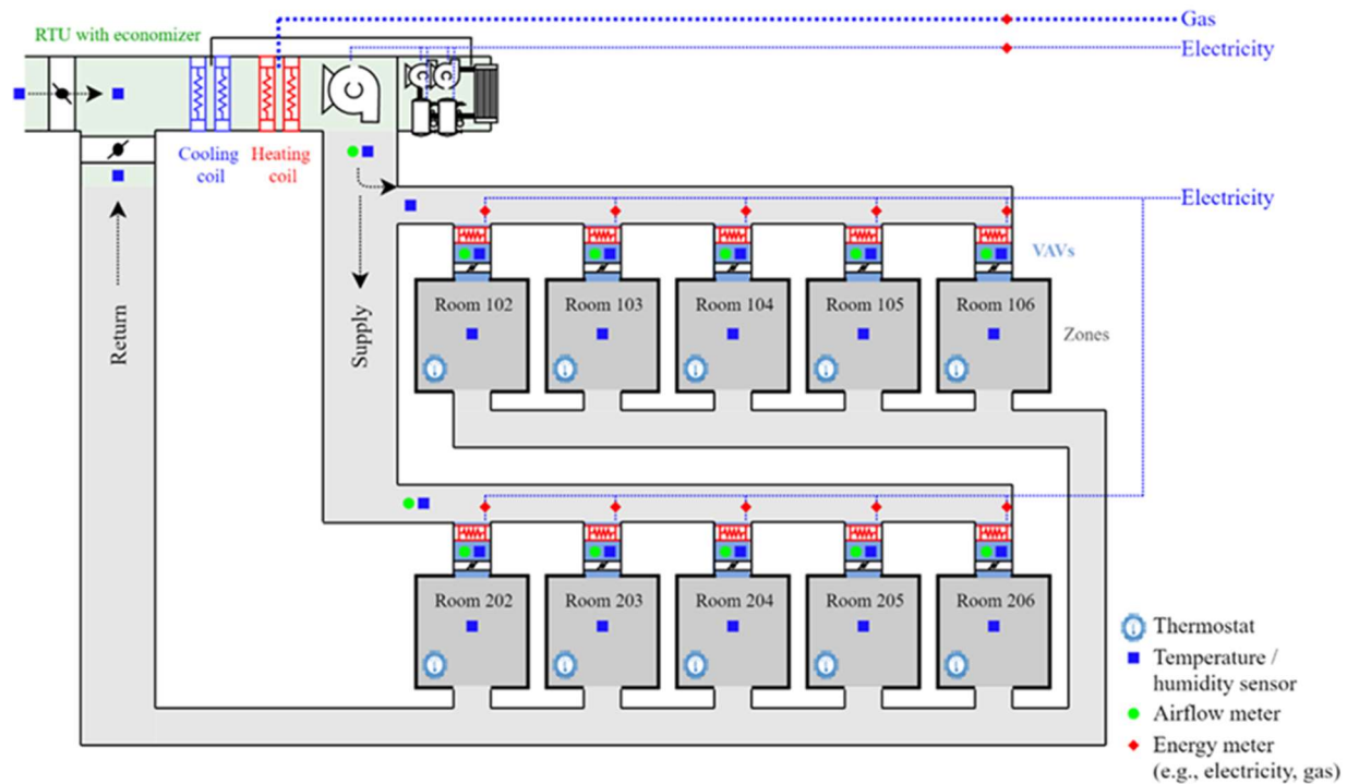
Figure 1. Variable air volume (VAV) centralized HVAC system configuration and measuring points
