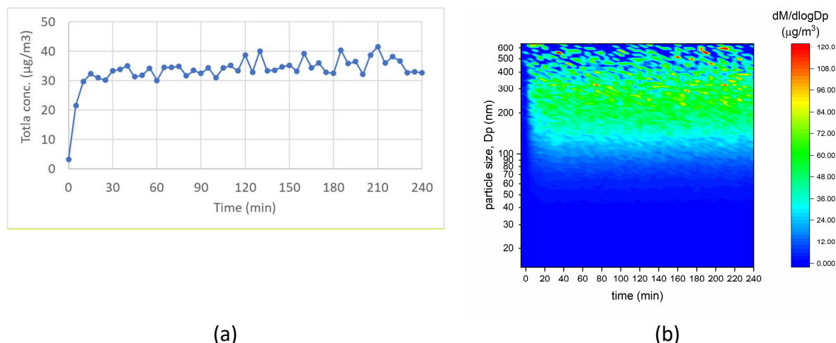
Figure 5. The total mass concentration (a) and size distribution over time (b) in the source room measuring sodium chloride testing aerosol using TSI model 3074 aerosol generator
