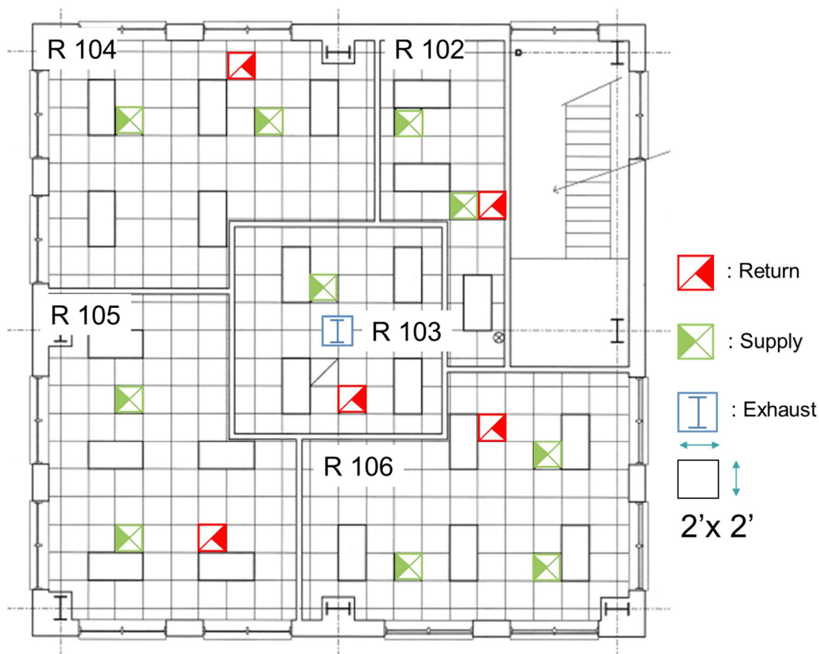
Figure 2. Locations of return, supply, and exhaust air on the first floor in the FRP
