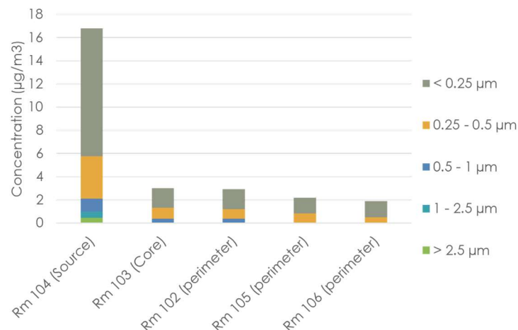
Figure 10. Aerosol concentrations under diffuser in the closed-door scenario
