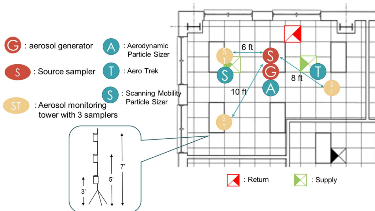
Figure 3. Location of samplers in the near-field campaign
