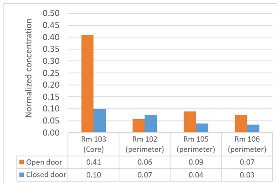
Figure 9. The spatial distribution of submicron normalized concentration
