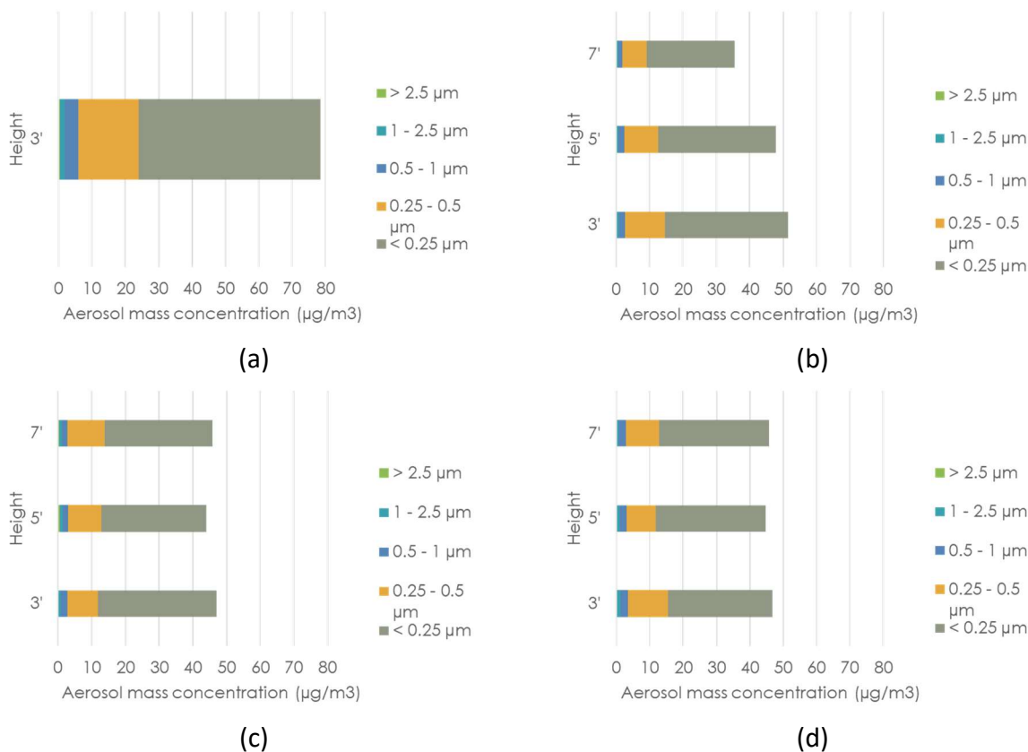
Figure 6. The spatial distribution of aerosol concentration measured at (a) source, (b) 6 ft, (c) 8 ft, and (d) 10 ft away from the source in the horizontal direction.
