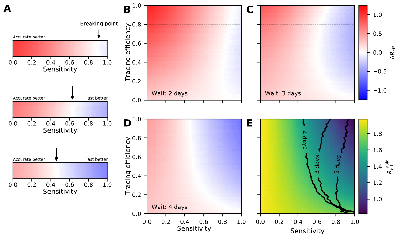
FIG. 2. A Comparison of effective reproduction number, \Delta R_{\text{eff}} = R_{\text{eff}}^{\text{slow}} - R_{\text{eff}}^{\text{rapid}} , when using a slow but accurate test with sensitivity 1 (no false negatives), and a test waiting time of \delta^{\text{slow}} days and using a rapid but less accurate test with a given sensitivity and test waiting time of \delta^{\text{rapid}} = 0 days. In this inset, we assume that 80% of secondary cases are successfully traced following a positive test. The colorbars show results obtained for different choices of \delta^{\text{slow}} (top colorbar: \delta^{\text{slow}} = 2 days, middle: \delta^{\text{slow}} = 3 days, bottom: \delta^{\text{slow}} = 4 days), and the rapid-test sensitivity (horizontal axis in each colorbar). In each colorbar a breaking point separates sensitivity values favoring the slower, accurate test and values favoring the rapid test. B Comparison of effective reproduction numbers when the result of the slower test arrives after \delta^{\text{slow}} = 2 days, as a function of the sensitivity and tracing efficiency. C Same as in B but with \delta^{\text{slow}} = 3 days. D Same as in B, C but with the slower result arriving after \delta^{\text{slow}} = 4 days. E Heatmap of the effective reproduction number obtained using the rapid, less accurate test, R_{\text{eff}}^{\text{rapid}} . The breaking-point lines of B, C, D are plotted in black.
