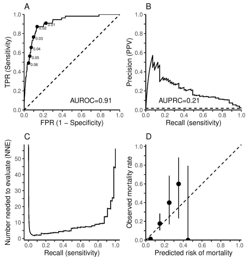
Figure 2. Performance metrics for in-hospital mortality in the test dataset. (A) Receiver operator characteristic plot, with labels indicating the corresponding threshold and the dashed line indicating the line of no discrimination. (B) Precision-recall plot, with the 1.8% observed incidence indicated by the dashed line. (C) Number needed to evaluate against sensitivity. (D) Calibration plot (with 95% CI), by tenths of predicted risk, with the dashed line indicating perfect calibration.
