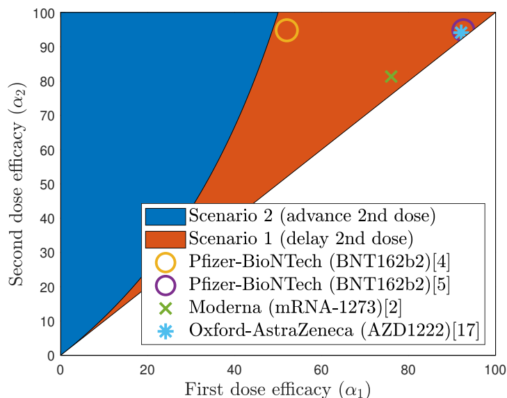
Figure 1: The answer to the question of delaying or advancing the second COVID-19 vaccine dose depends on the efficacies of each of the first and the second doses. This figure depicts the region (in red) where the best scenario would be to delay the second dose and the region (in blue) where the second dose should be advanced for optimal outcomes.
