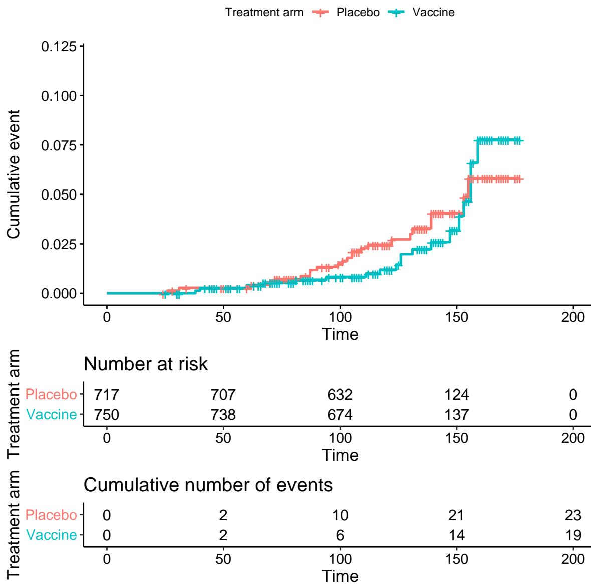
Figure 3: Kaplan-Meier plot of ChAdOx-1 nCoV19 against all-severity symptomatic Covid-19 illness following two doses versus placebo.
