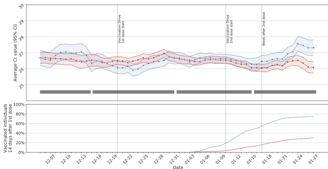
Figure 1: The Ct value distribution as a function of date. Blue: 60+ individuals. Red: Individuals between the ages of 40-60yrs. Upper: the average Ct value of positive tests per age group smoothed using a 7 day rolling window. The shadowed area shows the 95% confidence interval. The gray rectangles represent the four comparison periods in Figure 2 . The nationwide percentage of individuals who are 14 days after receiving their first dose [data processed from the Ministry of Health dashboard].
