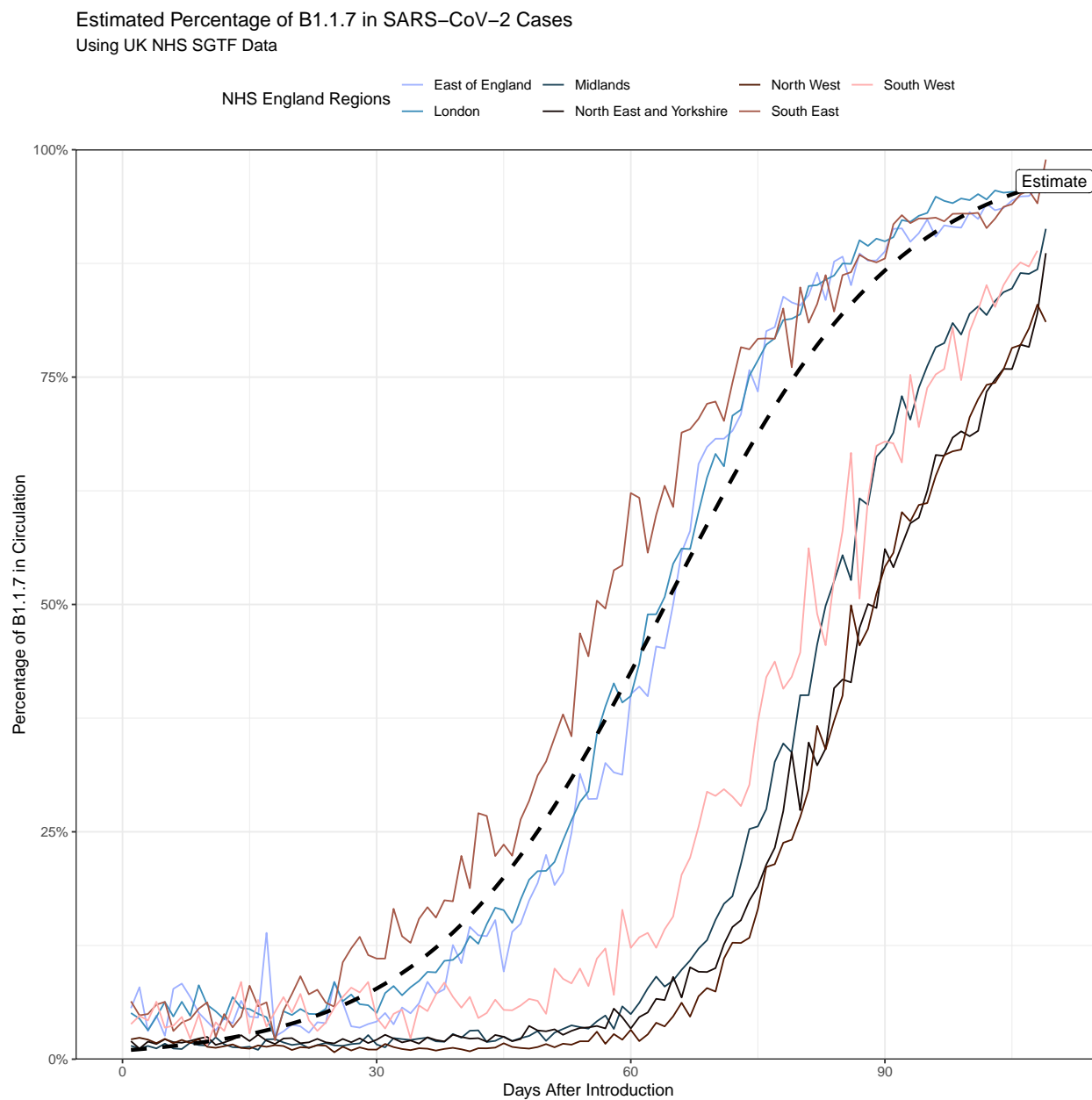
Figure 1: Estimates of SGTF Evolution Used as Proxy for B1.1.7 Share of SARS-CoV-2 Variants in Circulation
