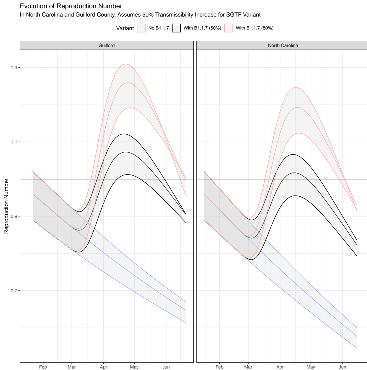
Figure 2: Estimates of Reproduction Number Evolution in North Carolina and Guilford County Shows Heterogeneity
