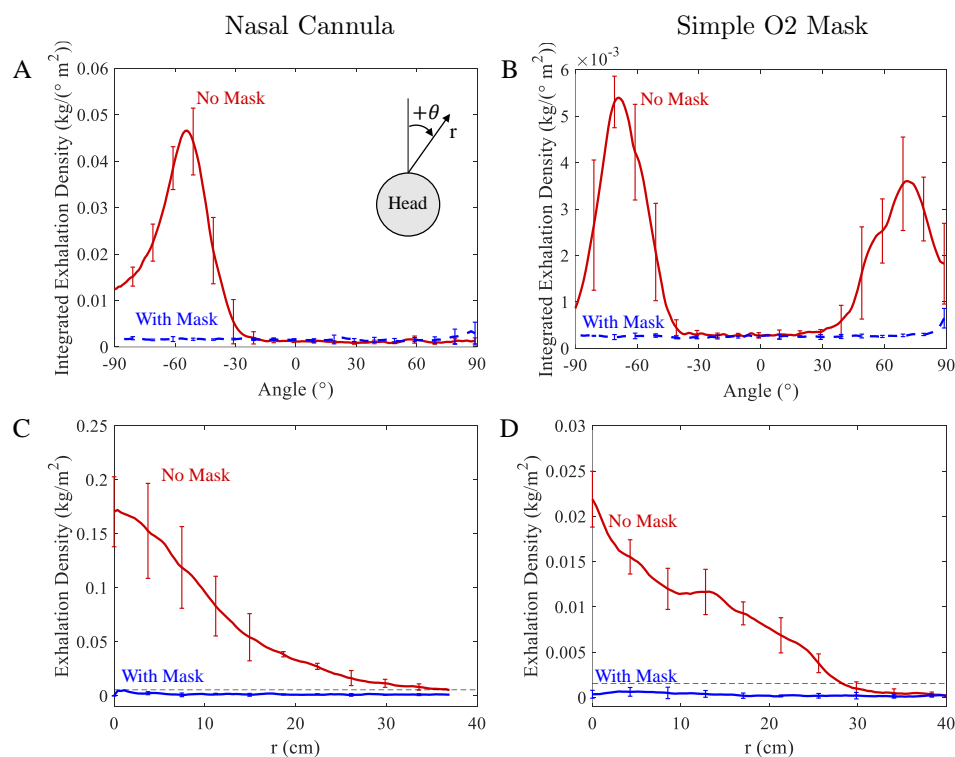
Figure 4: The angular integrated dispersal exhalation intensity is suppressed when a surgical mask is placed on top in both devices (A,B). The distance over which the jets reach is observed to be dramatically curtailed in both devices (C,D). The bars represent the range of values among five trials used to calculate the plotted averages. The exhalations travel up to 37 cm for the nasal cannula and 31 cm for the simple O 2 mask when unmitigated. The black dashed line represents the threshold value that is 50% greater than the mean exhalation density \rho_m used to determine the exhalation distance.
