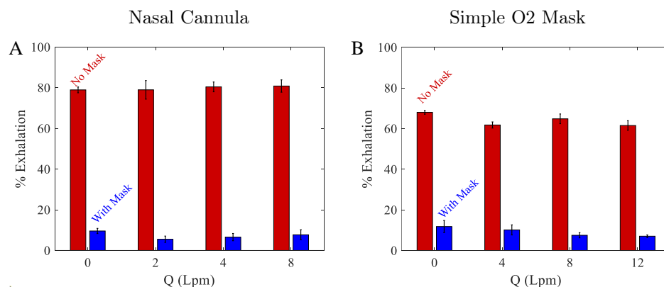
Figure 5: The percent of breath that is exhaled above the face without and with surgical mask as a function of flow rates for (A) the nasal cannula and (B) the simple O 2 mask. All cases have five trials.
