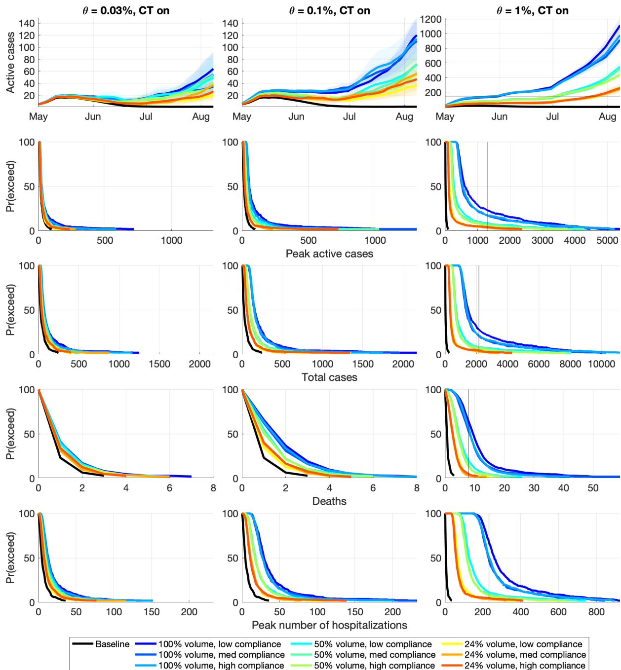
Figure 3: Simulation outcomes with contract tracing (CT). 95% confidence intervals are shown, and the mean is bolded. \theta is the traveller infection rate. Note that \theta = 1\% is on a different scale; the horizontal line at \approx 140 cases in \theta = 1\% active cases (top) indicates the upper limit of the figures for \theta = 0.03\% and 0.1\% , while the vertical lines in other rows indicate the maximum x -axis value for \theta = 0.03\% and 0.1\% .
