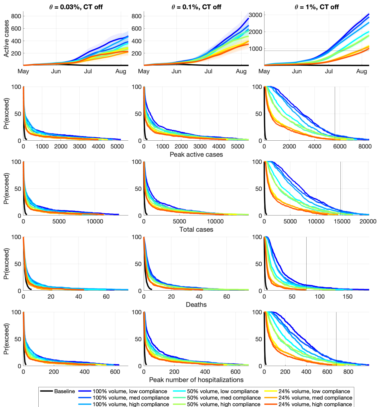
Figure 2: Simulation outcomes without contract tracing (CT). 95% confidence intervals are shown, and the mean is bolded. \theta is the traveller infection rate. Note that \theta = 1\% is on a different scale; the horizontal line at \approx 800 cases in \theta = 1\% active cases (top) indicates the upper limit of the figures for \theta = 0.03\% and 0.1\% , while the vertical lines in other rows indicate the maximum x -axis value for \theta = 0.03\% and 0.1\% .
