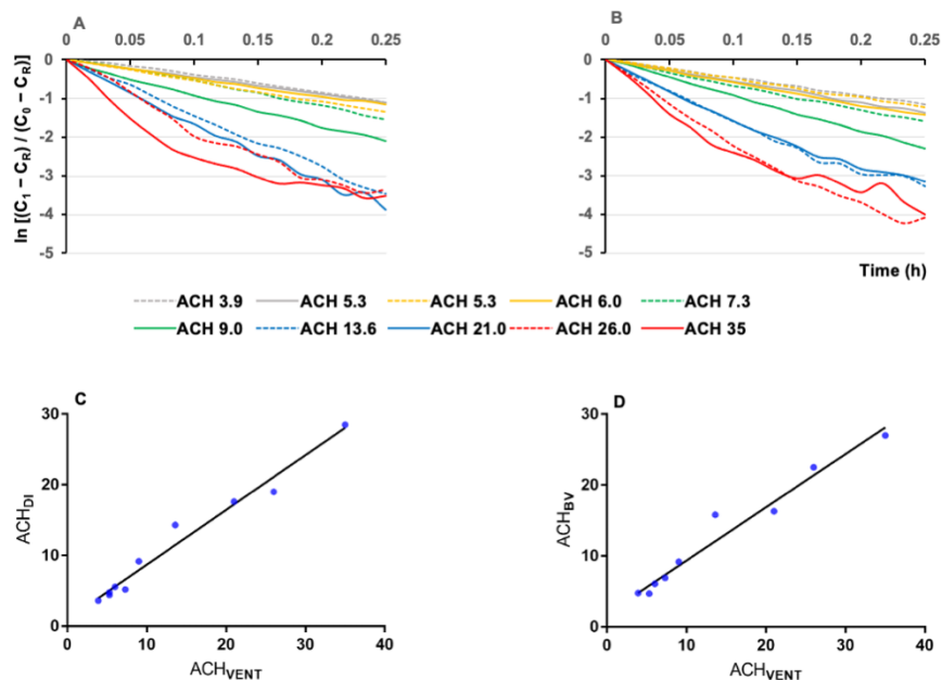
Figure 3. A: CO 2 decay constants by dry ice, B: CO 2 decay constants by baking soda and vinegar; C and D: association between mechanical ventilation rates measure by air flow ( ACH_{VENT} ) and ventilation rates measured by CO 2 decay using dry ice ( ACH_{DI} ) and baking soda and vinegar ( ACH_{BV} ) in dental treatment rooms. Rooms with high mechanical ventilation rates showed rapid decrease of CO 2 concentrations over time (A, B). Both ACH_{DI} and ACH_{BV} are linearly correlated with ACH_{VENT} (C, D).
