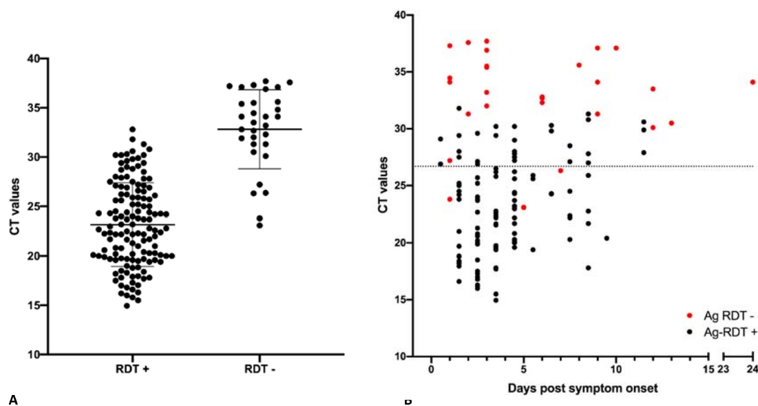
Figure 1. SARS-CoV-2 detection by Panbio™ antigen rapid test using OPS compared to the reference RT-qPCR detection method using NPS. A. Ct values, viral load and Ag-RDT results for 166 RT-PCR-positive individuals. Horizontal bars represent median and standard deviation. Dotted line: Ct value of 26.7 or 1E6 SARS-
