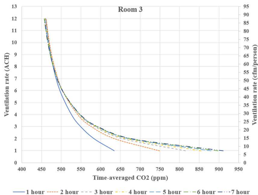
1 Fig. 5 Relation of indoor CO 2 levels and ventilation rates for classrooms.
