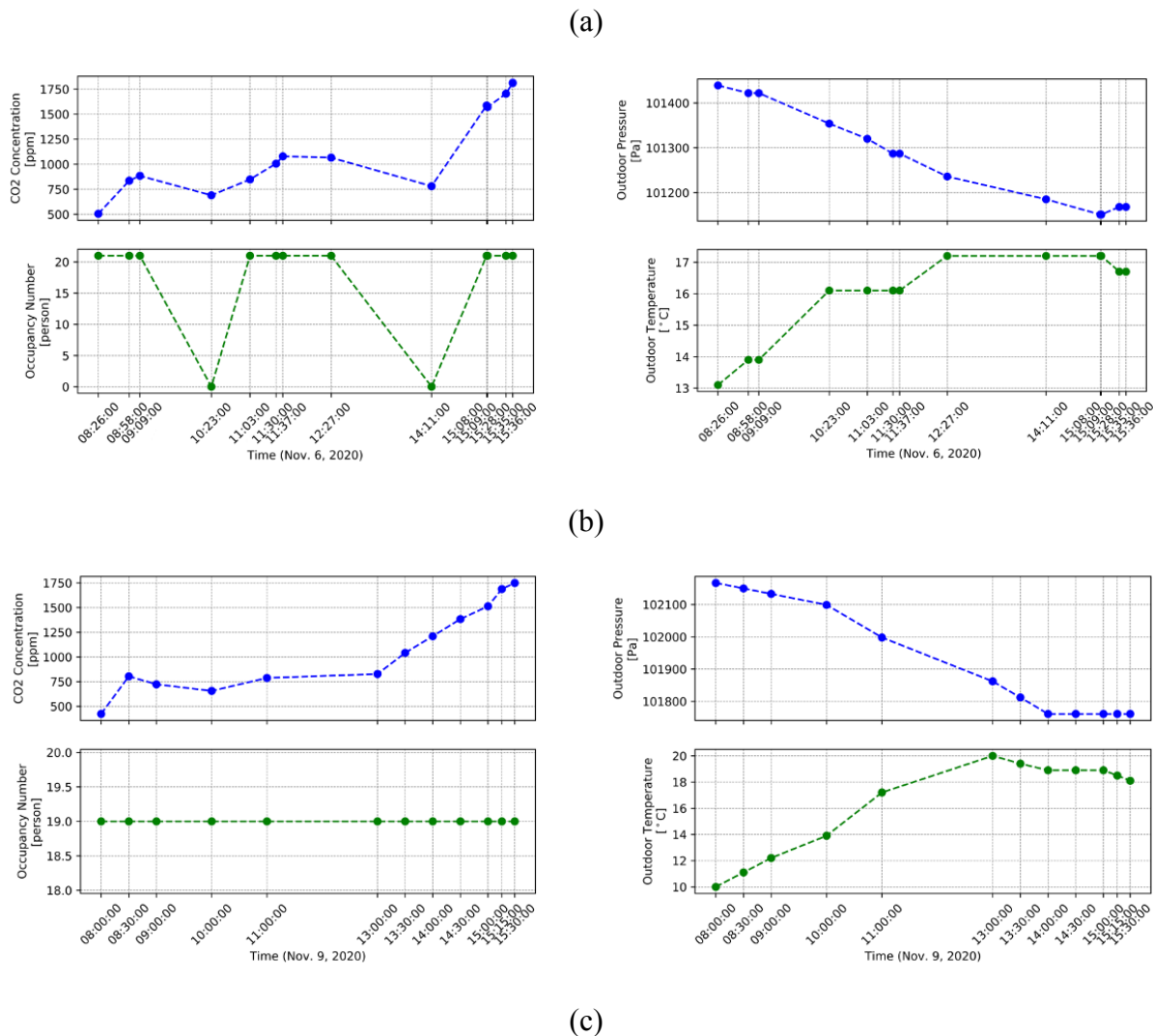
1 Fig. 2 CO 2 concentration measurements, occupancy number profile, outdoor air temperature, and 2 outdoor air pressure of a) Room 1, b) Room 2, c) Room 3.
