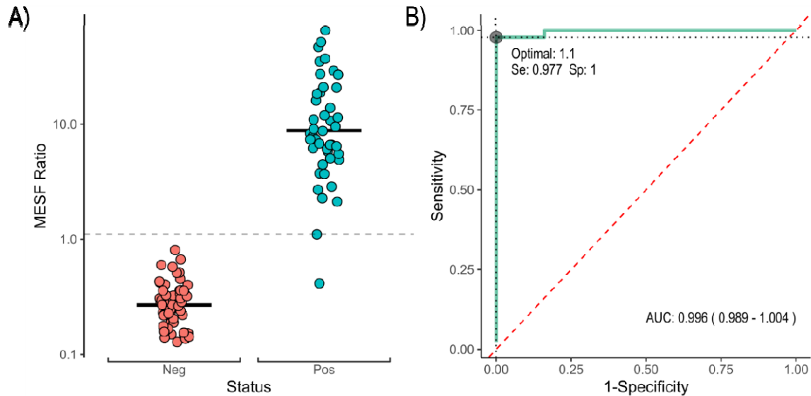
Figure 1: (A) Distribution of MESF ratios relative to CR3022 (50 ng/ml) control for pre-COVID (Neg, red dots), n=56 , and convalescent plasmas (Pos, green dots), n=44 . The dotted line represents the positivity threshold. Black bars are the means for each group (0.30 and 13.95 for negative and positive groups respectively). (B) ROC curve (green) and optimal threshold point determined by Youden's index. The red dashed line is the line of no discrimination.
