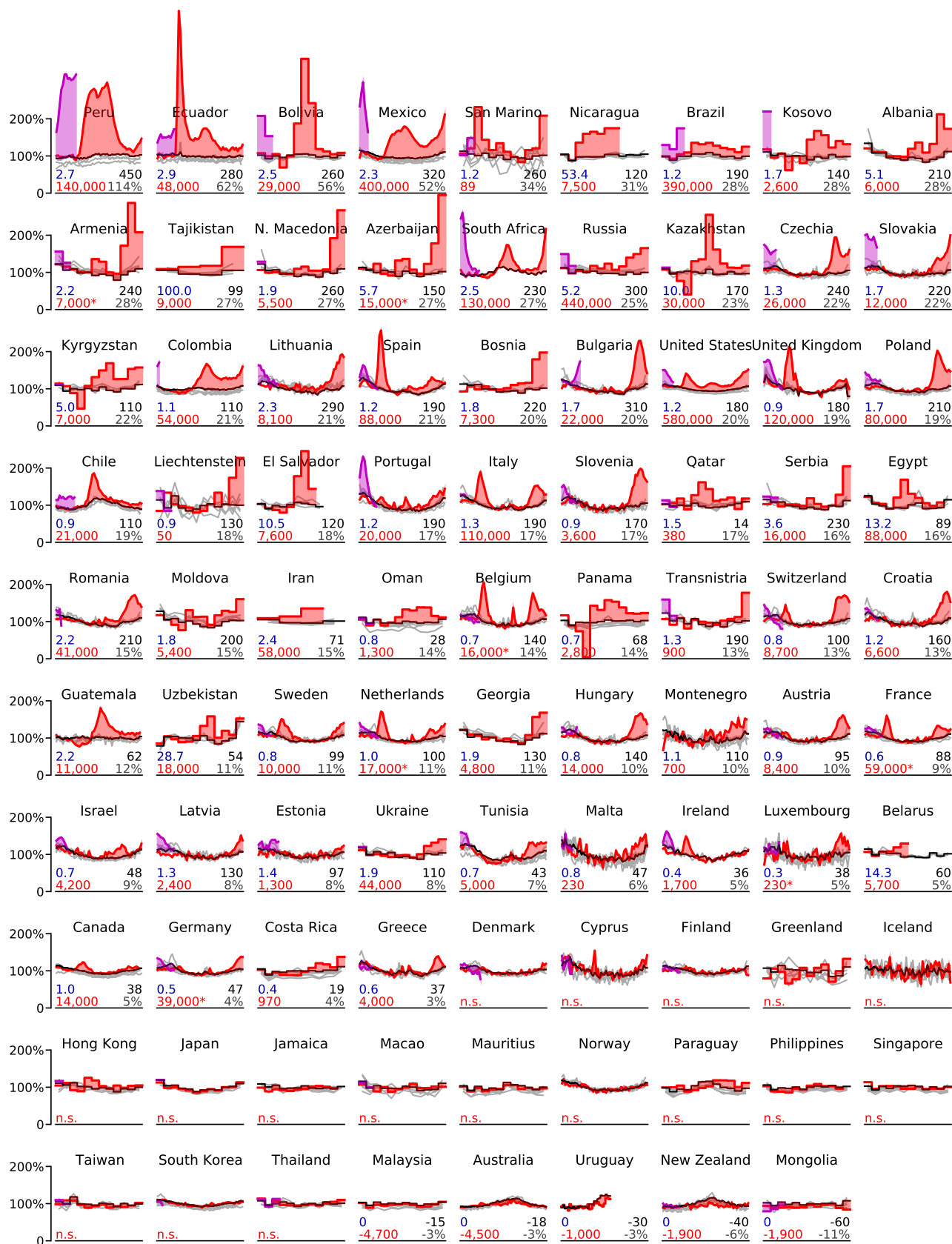
Figure 2: Excess mortality time series. Each subplot shows baseline mortality (black), mortality in 2015–2019 (gray), in 2020 (red) and in 2021 (purple). Excess mortality is shown in red/purple shading. The numbers in each subplot are: total excess mortality (red), excess mortality per 100,000 population (black), excess mortality as a percentage of annual baseline mortality (gray), and undercount ratio of COVID-19 deaths (blue). See text for the exact definitions. “n.s.” – excess mortality not significantly different from zero ( t < 2 ). All numbers were rounded to two significant digits. The y -axis in each subplot starts at 0 and goes until 200% where 100% corresponds to the average baseline mortality. The x -axis covers the entire year. Asterisks mark excess mortality estimates that were downwards corrected (see Methods). Countries are sorted by the excess mortality as a percentage of annual baseline mortality (gray number).
